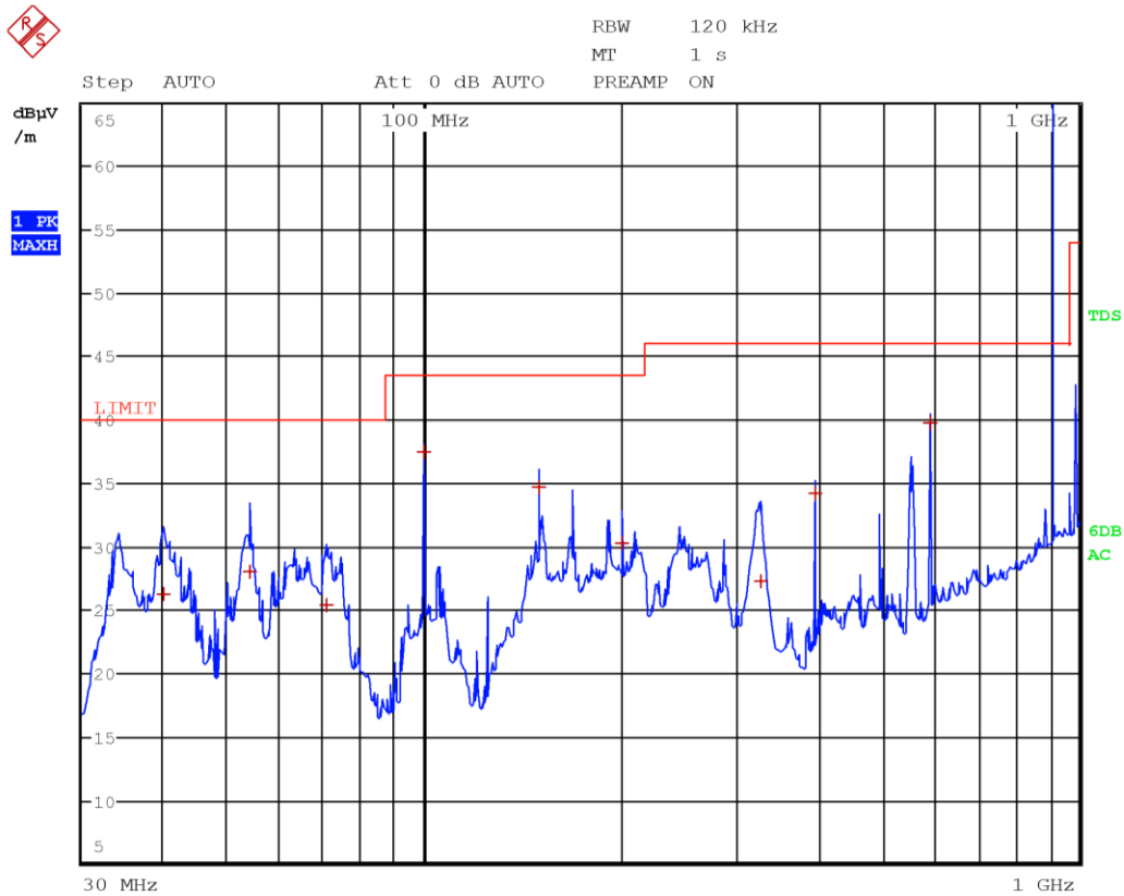
Radiated spurious emissions with antenna in vertical polarization and with WCDMA Tx at 1880 MHz, UHF Tx at 915 MHz, WIFI Tx at 5220 MHz and BT Tx at 2441 MHz (antenna configuration 1)
