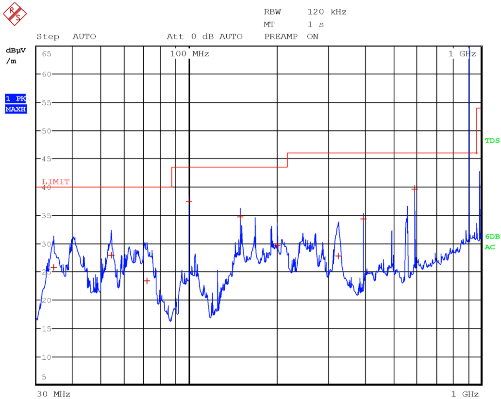
Radiated spurious emissions with antenna in vertical polarization and with WCDMA Tx at 1880 MHz, UHF Tx at 915 MHz, WIFI Tx at 2437 MHz and BT Tx at 2441 MHz (antenna configuration 1)
