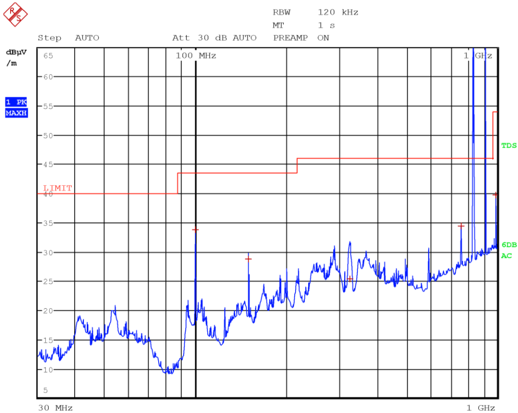
Radiated spurious emissions with antenna in horizontal polarization and with WCDMA Tx at 837 MHz, UHF Tx at 915 MHz, WIFI Tx at 2437 MHz and BT Tx at 2441 MHz (antenna configuration 1)
