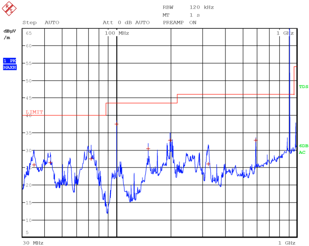
Radiated spurious emissions with antenna in vertical polarization and with LTE Tx at 1732.5 MHz, UHF Tx at 915 MHz, WIFI Tx at 5220 MHz and BT Tx at 2441 MHz (antenna configuration 2)
