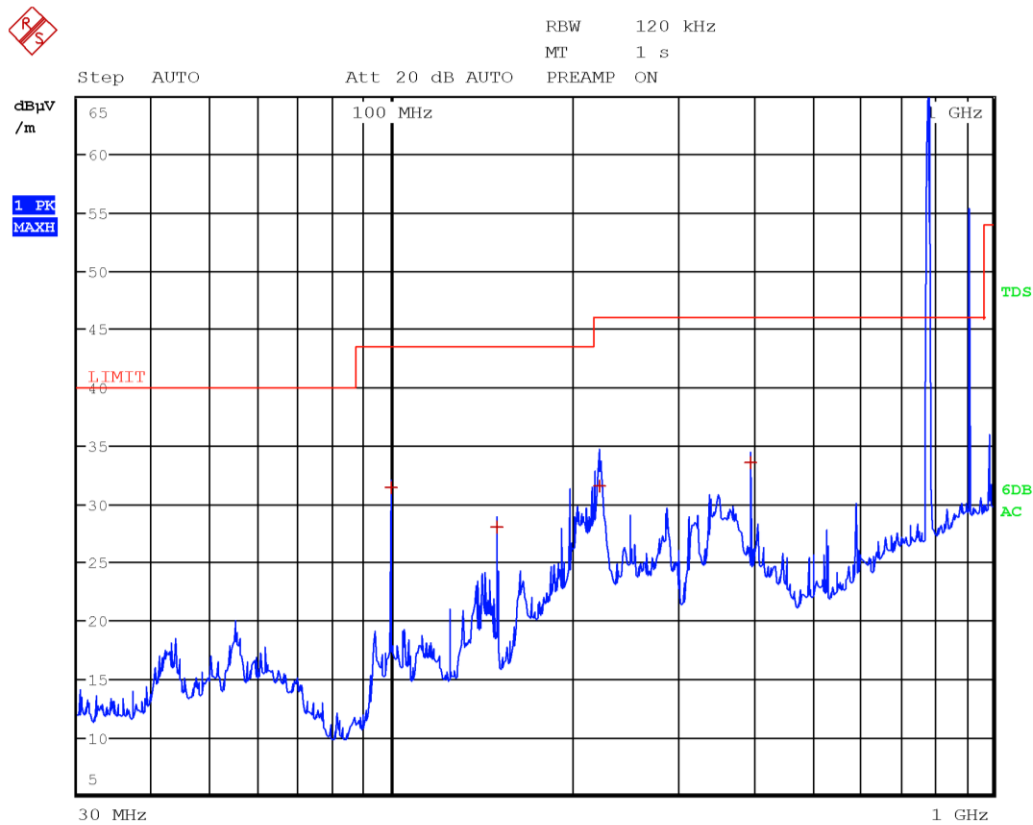
Radiated spurious emissions with antenna in horizontal polarization and with LTE Tx at 782 MHz, UHF Tx at 915 MHz, WIFI Tx at 2437 MHz and BT Tx at 2441 MHz (antenna configuration 2)
