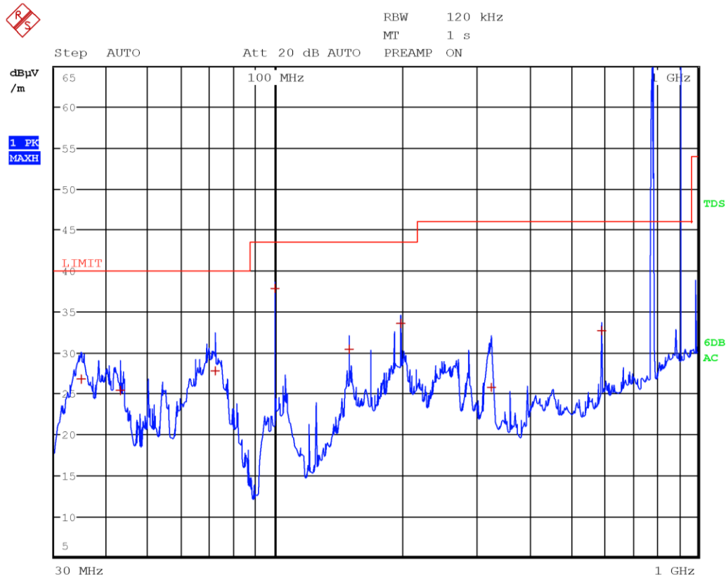
Radiated spurious emissions with antenna in vertical polarization and with LTE Tx at 782 MHz, UHF Tx at 915 MHz, WIFI Tx at 2437 MHz and BT Tx at 2441 MHz (antenna configuration 2)
