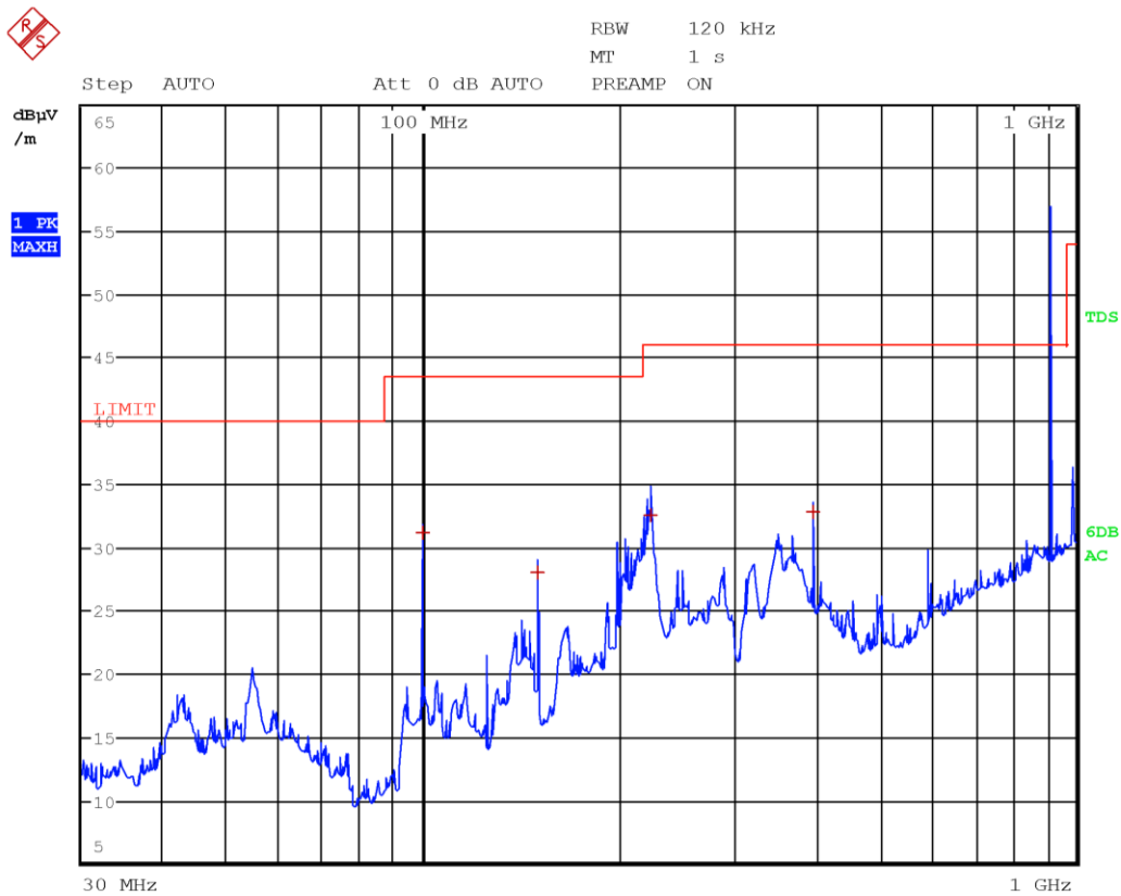
Radiated spurious emissions with antenna in horizontal polarization and with LTE Tx at 1732.5 MHz, UHF Tx at 915 MHz, WIFI Tx at 2437 MHz and BT Tx at 2441 MHz (antenna configuration 2)
