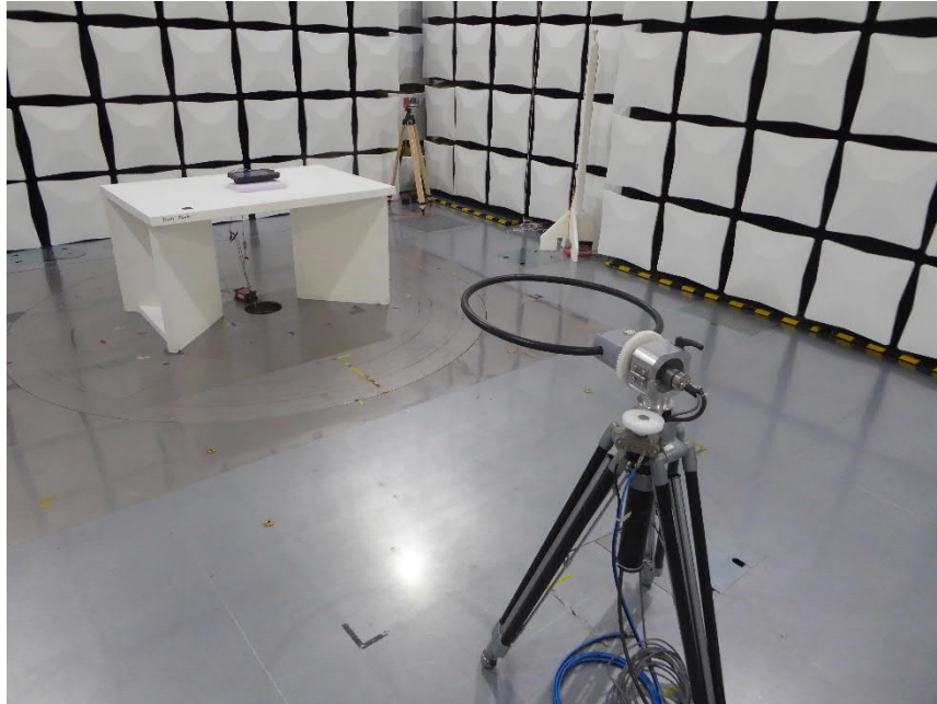
EUT Position 3 – lying / Antenna Position 3 – grund-parallel Test setup semi-anechoic chamber M276 Preliminary measurement
