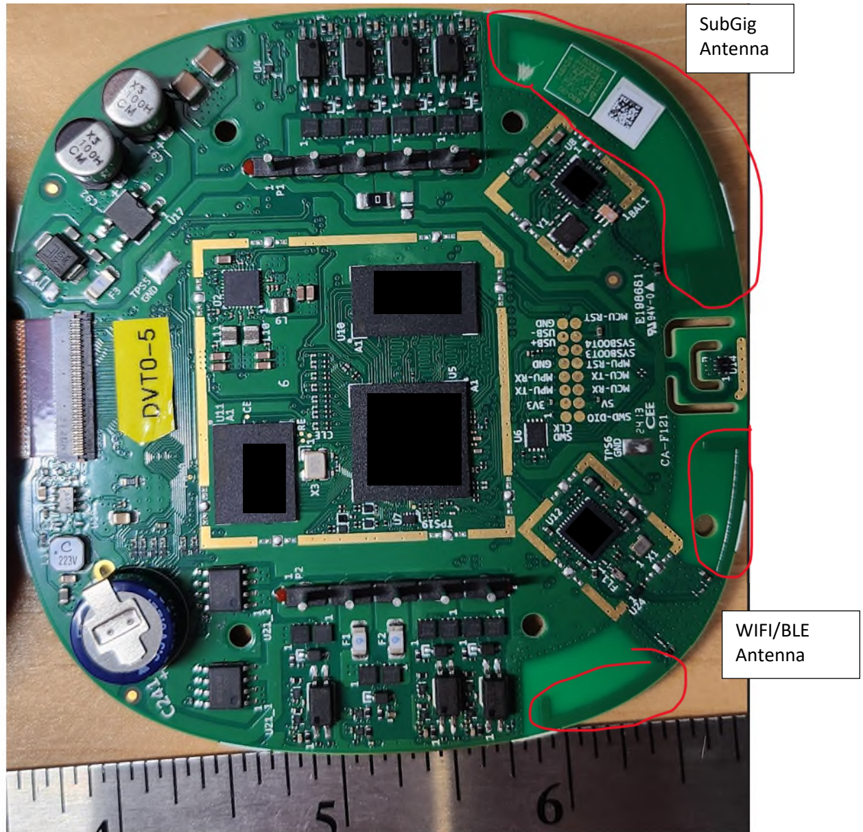
Figure 3 – Smart Thermostat Lite – PCB Top
