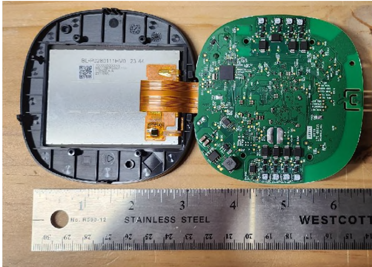
Figure 1 – Smart Thermostat Lite/Essential – PCB Bottom with display View
