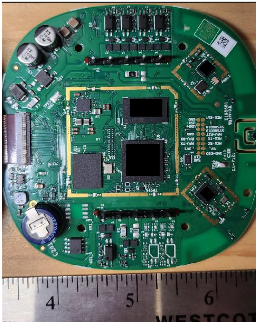
Figure 4 – Smart Thermostat Essential – PCB Top
