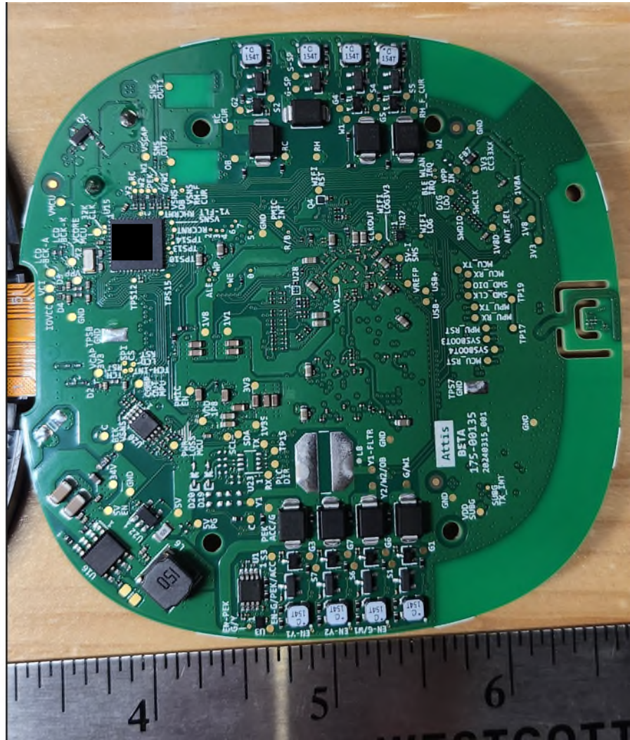
Figure 2 – Smart Thermostat Lite/Essential – PCB bottom
