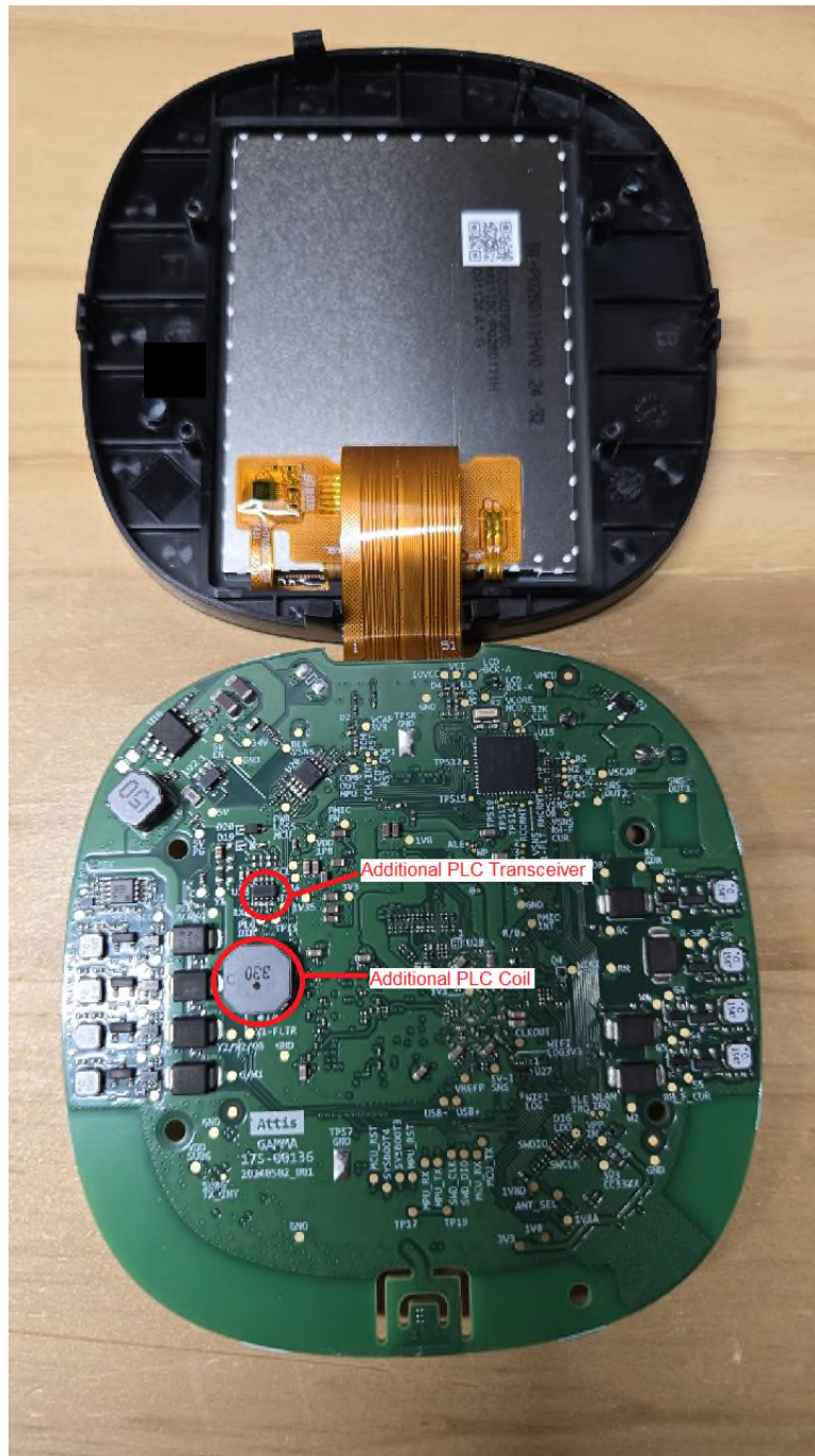
Figure 1 – Smart Thermostat Lite – PCB bottom
