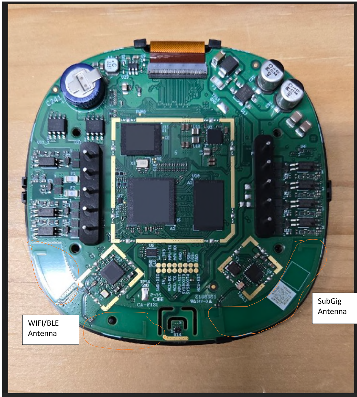
Figure 3 – Smart Thermostat Lite – PCB Top
