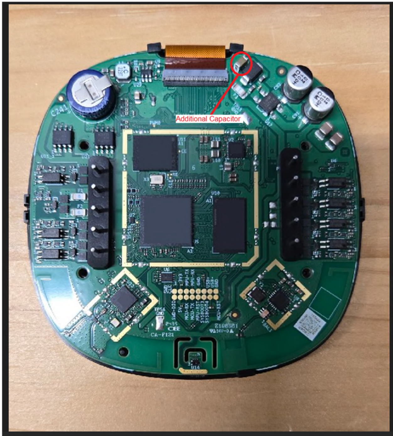
Figure 2 – Smart Thermostat Lite – PCB Top
