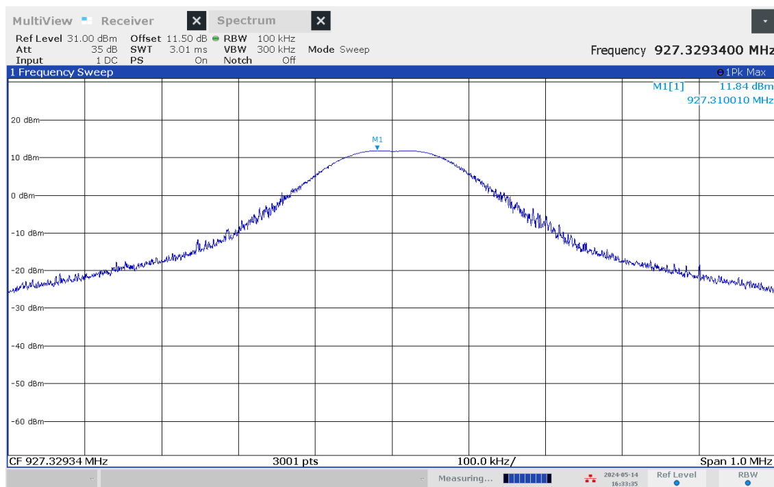
Figure 12 – -20dBc Reference Level - High Channel
