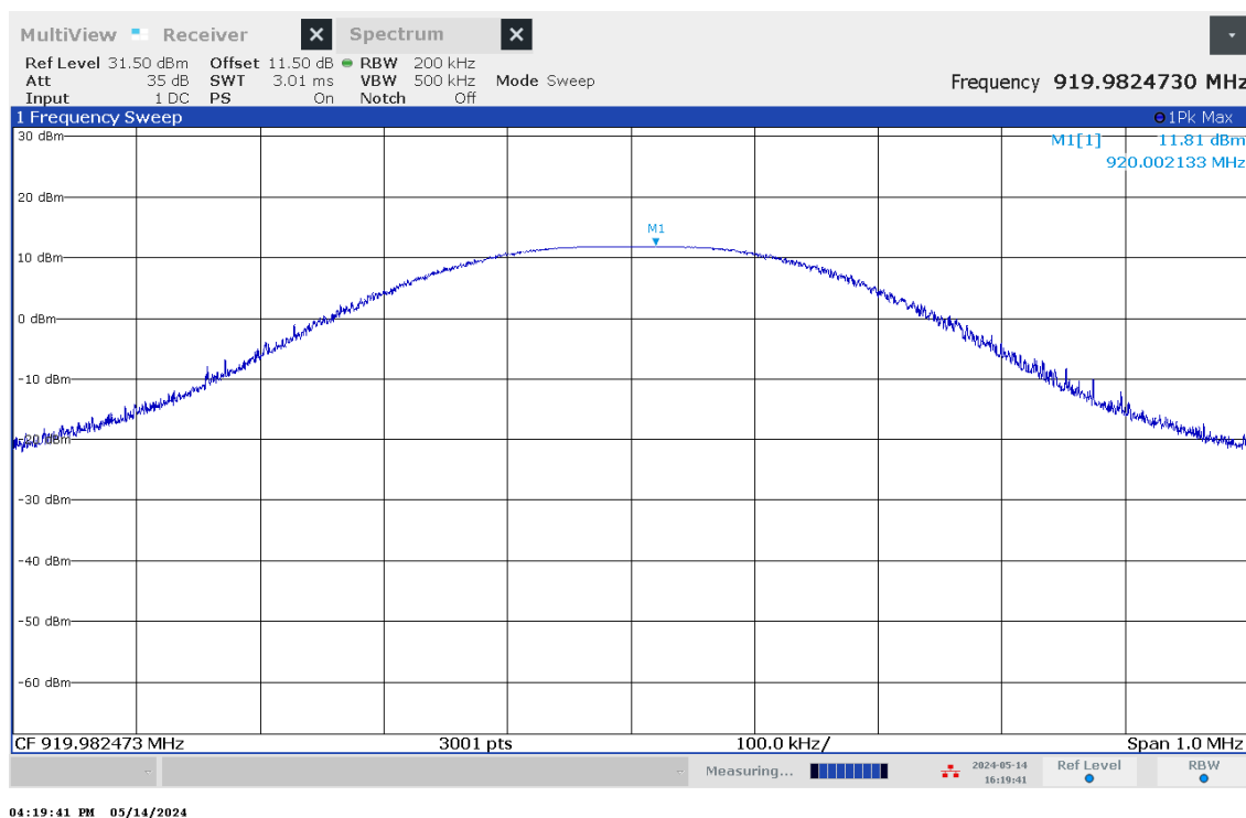
Figure 10 – Peak Power - Low Channel
