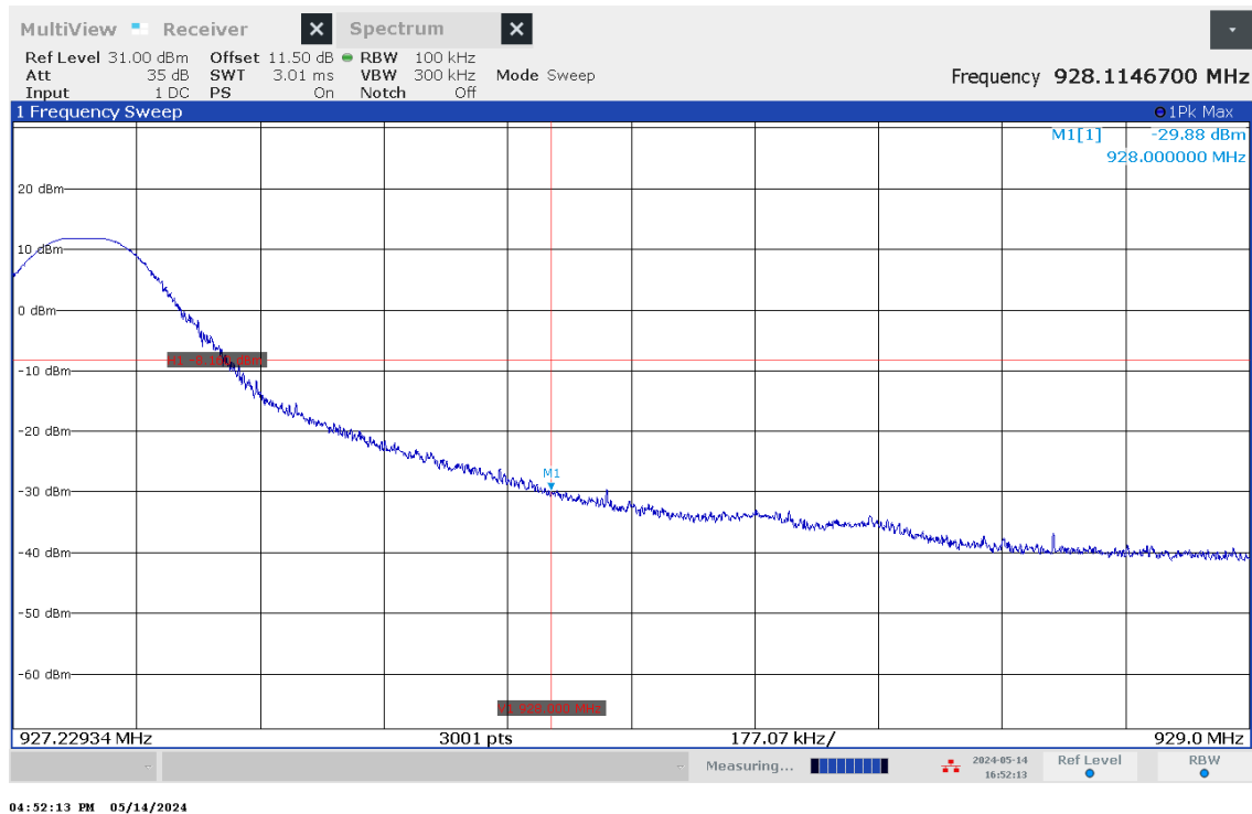
Figure 16 – -20dBc Band Edge - High Channel (Hoping Disabled)
