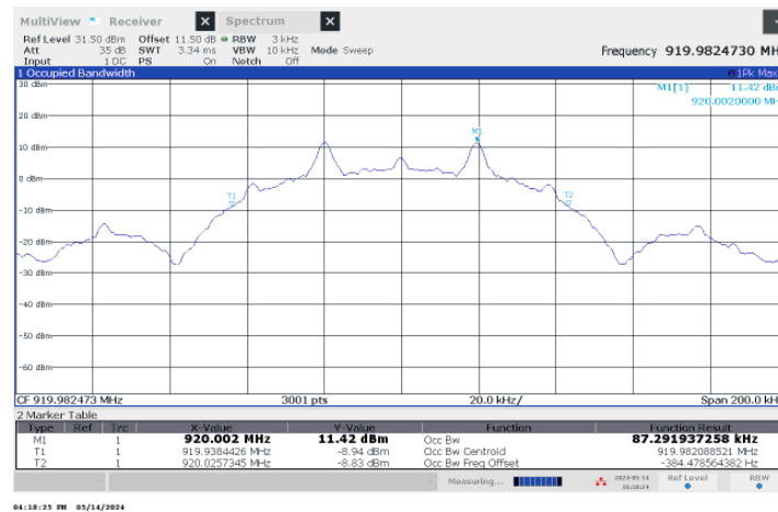
Figure 4 – 99% Bandwidth - Low Channel
