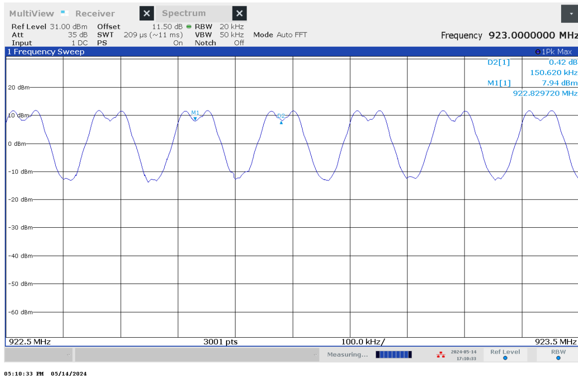
Figure 6 – Channel Separation
