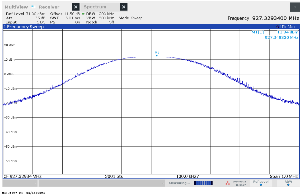
Figure 11 – Peak Power - High Channel
