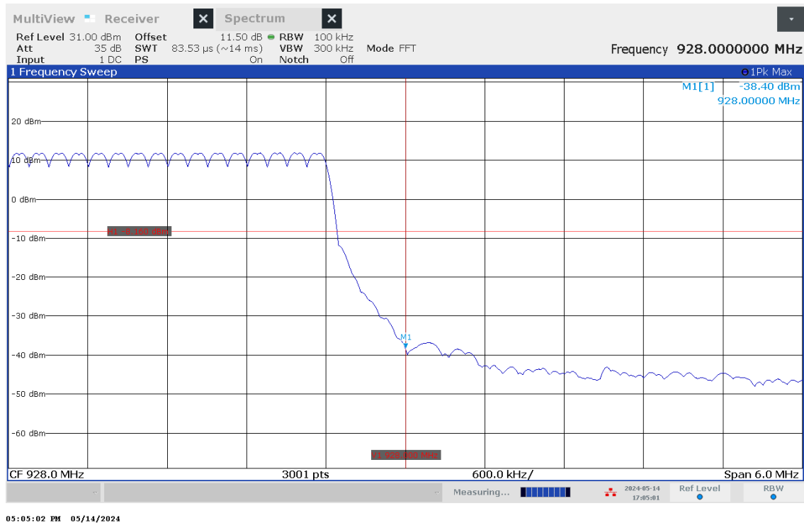
Figure 17 – -20dBc Band Edge - High Channel (Hoping Enabled)
