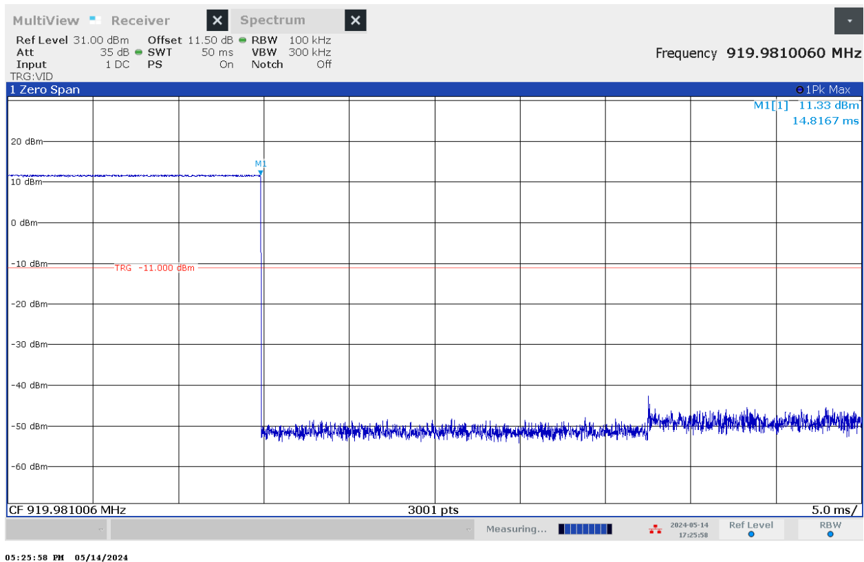
Figure 8 – Dwell Time per Hop
