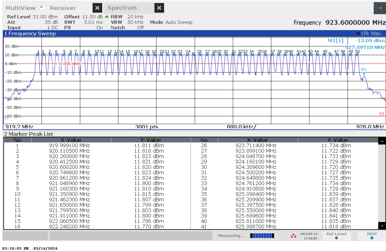
Figure 7 – Number of Hopping Channels
