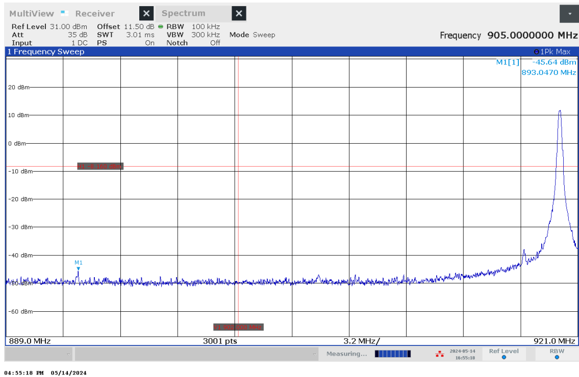
Figure 14 – -20dBc Band Edge - Low Channel (Hoping Disabled)
