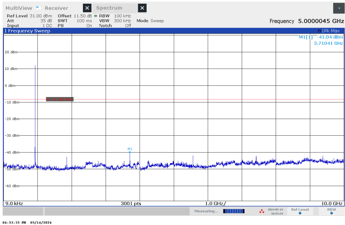
Figure 13 – -20dBc with High Channel
