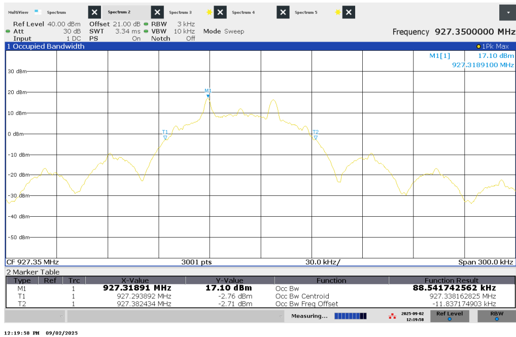
Figure 5 – 99% Bandwidth - High Channel
