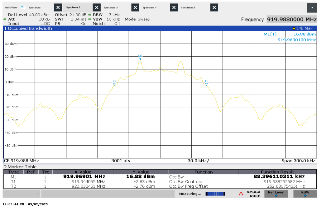
Figure 4 – 99% Bandwidth - Low Channel
