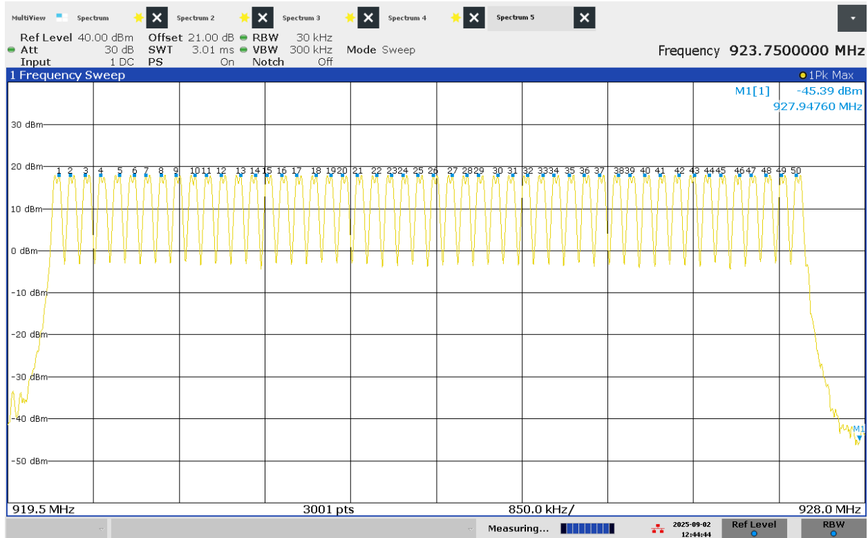
Figure 7 – Number of Hopping Channels
