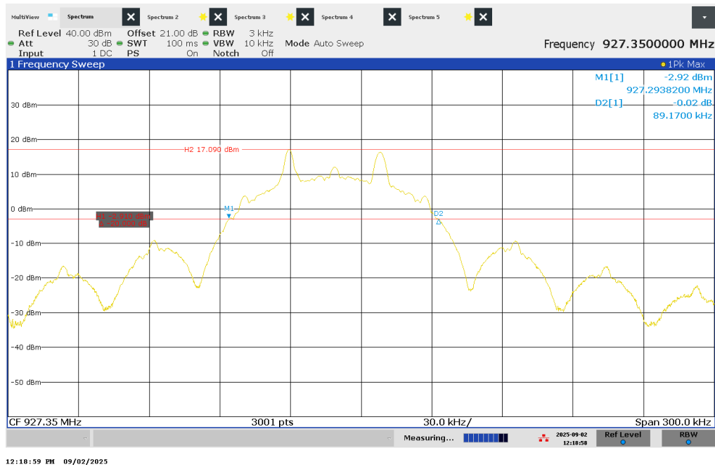
Figure 3 – 20 dB Bandwidth - High Channel
