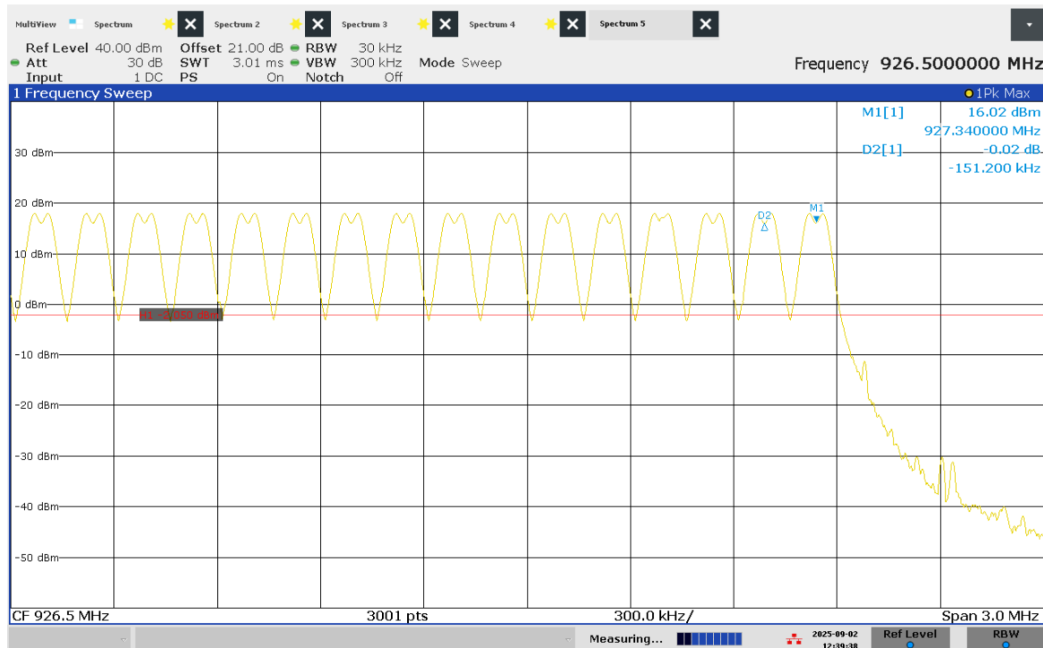
Figure 6 – Channel Separation
