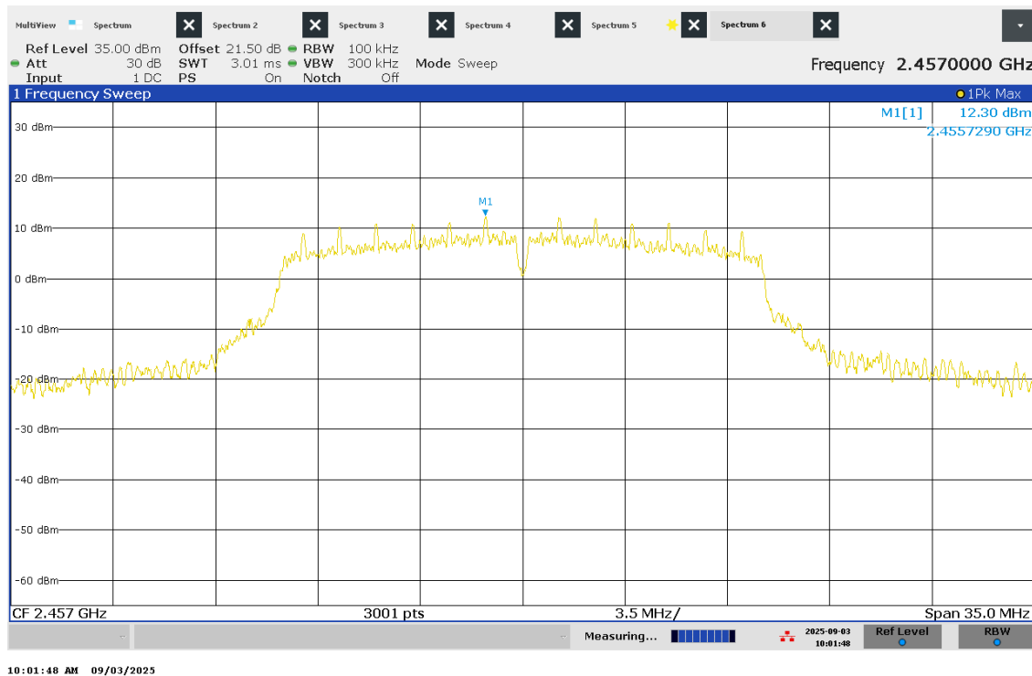
Figure 60 – -30dBc Reference Level
