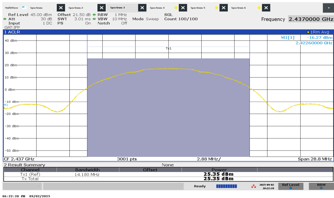
Figure 27 – Average Power - Mid Channel
