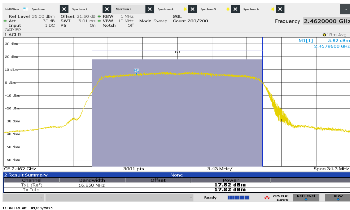
Figure 33 – Average Power – Channel 11
