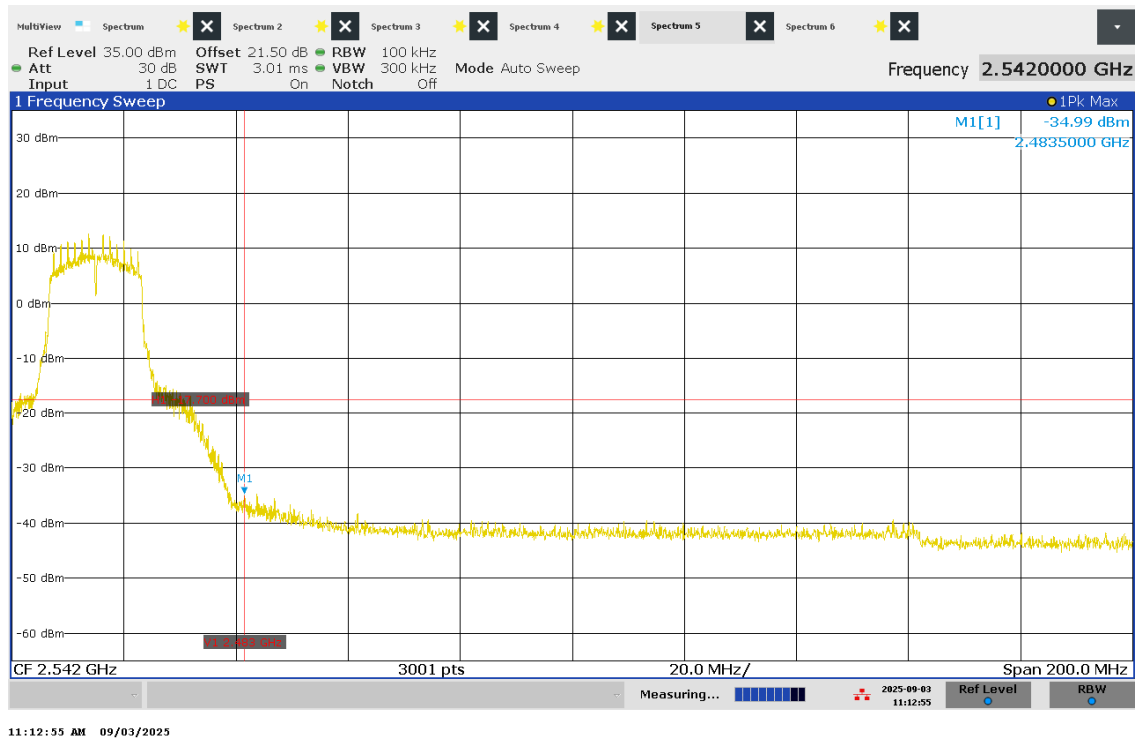
Figure 63 – -30dBc Band Edge – Channel 10
