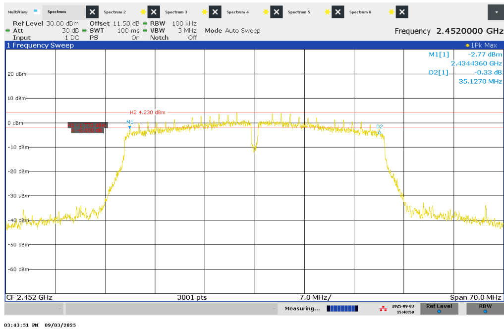
Figure 22 – 6dB Bandwidth – 2452 MHz
