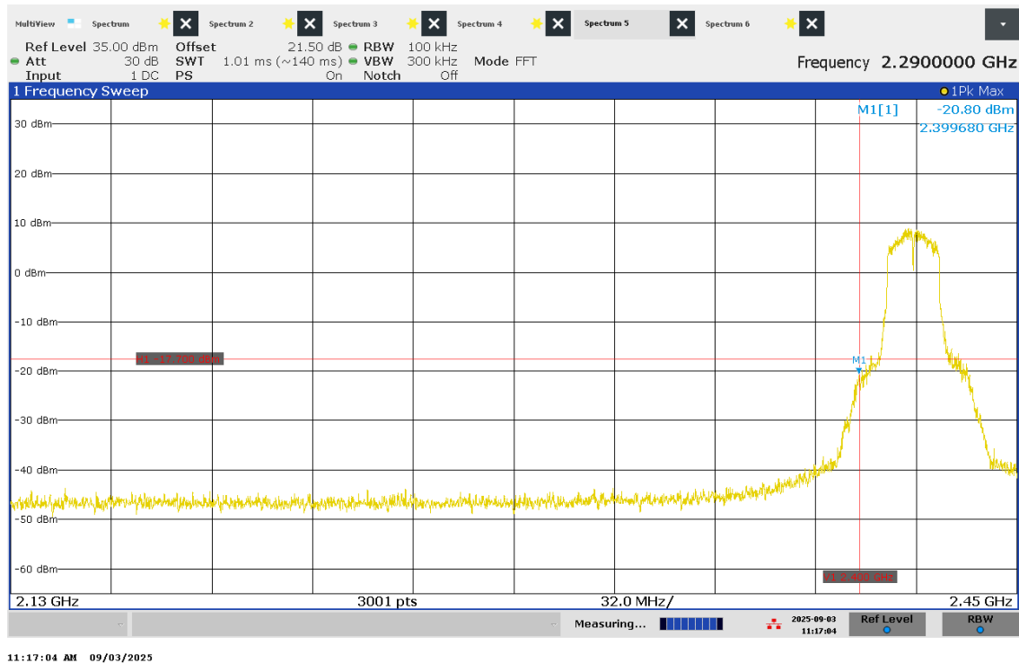
Figure 62 – -30dBc Band Edge – Channel 2
