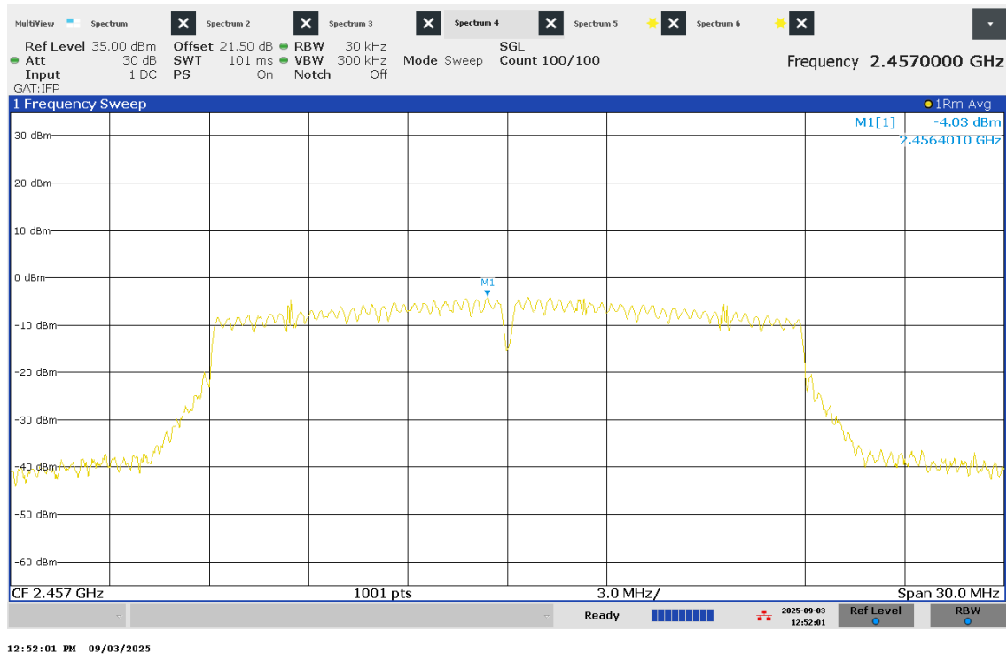
Figure 51 – PSD – Channel 10
