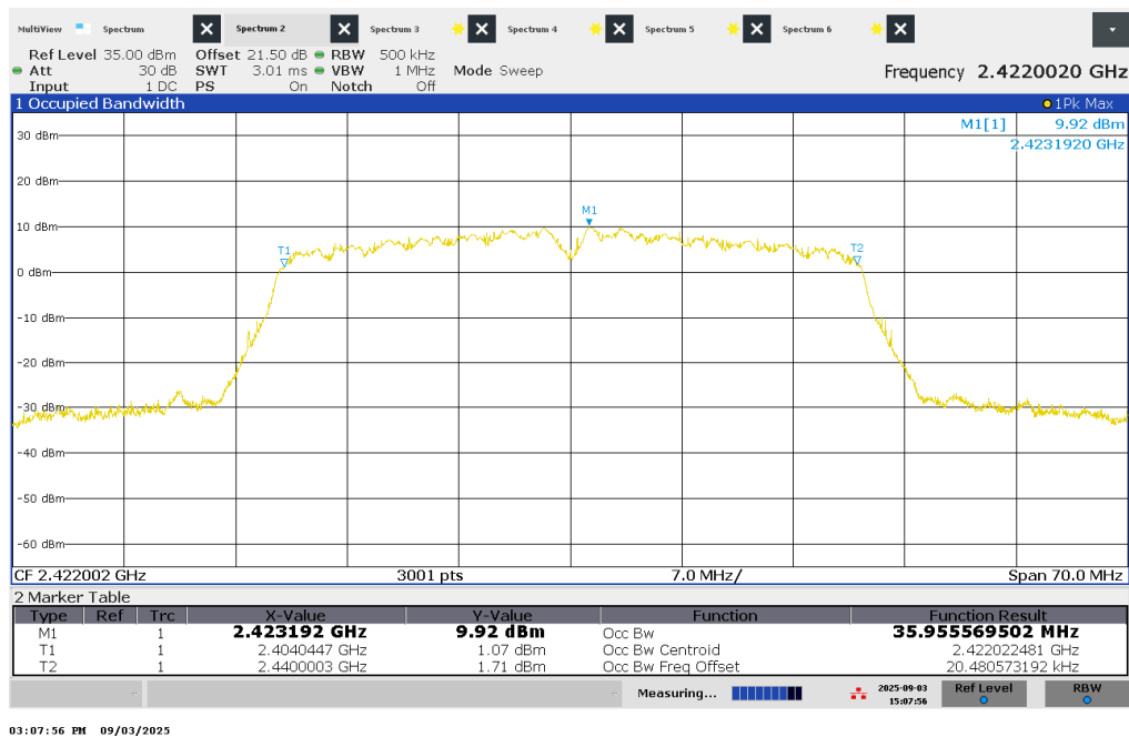
Figure 23 – 99% Bandwidth – 2422 MHz
