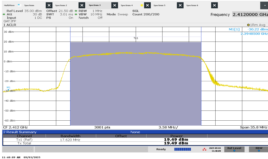
Figure 34 – Average Power - Low Channel
