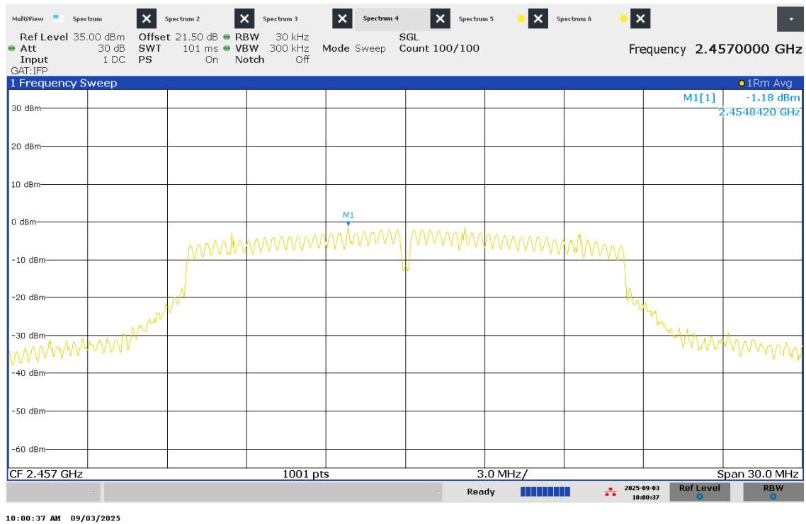
Figure 47 – PSD – Channel 10
