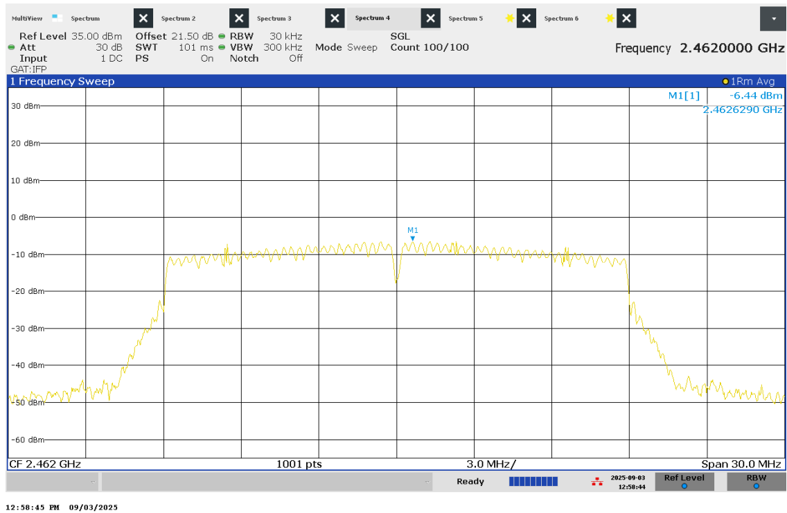
Figure 52 – PSD – Channel 11
