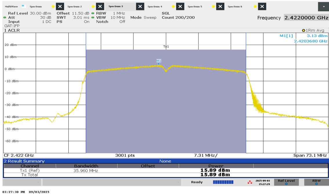
Figure 38 – Average Power - Low Channel
