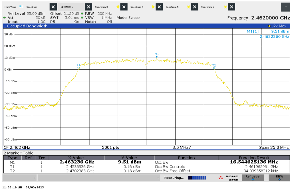
Figure 13 – 99% Bandwidth – 2462 MHz
