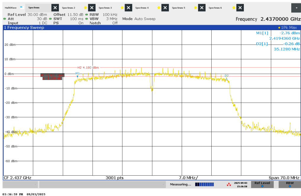
Figure 21 – 6dB Bandwidth – 2437 MHz
