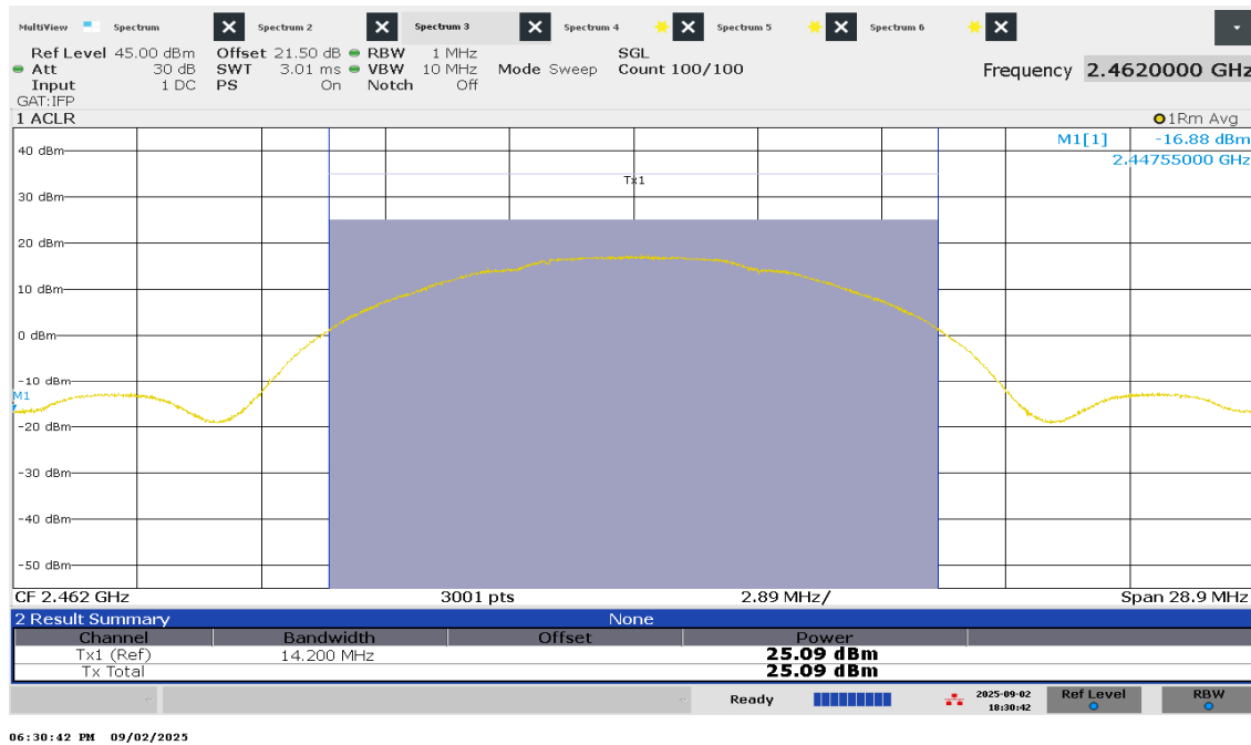
Figure 28 – Average Power - High Channel
