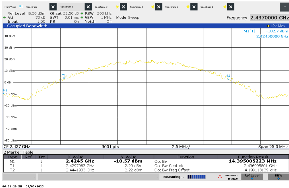
Figure 6 – 99% Bandwidth – 2437 MHz
