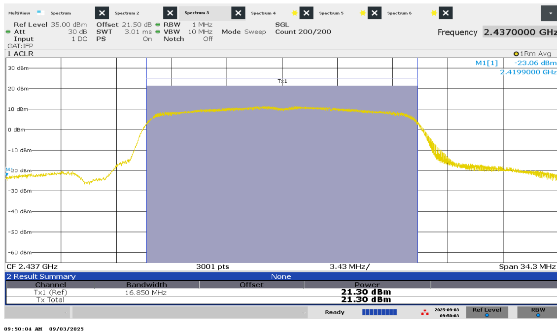
Figure 31 – Average Power - Mid Channel
