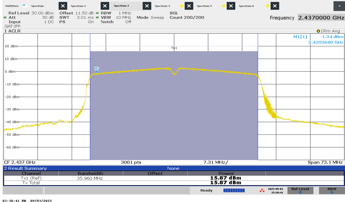
Figure 39 – Average Power - Mid Channel
