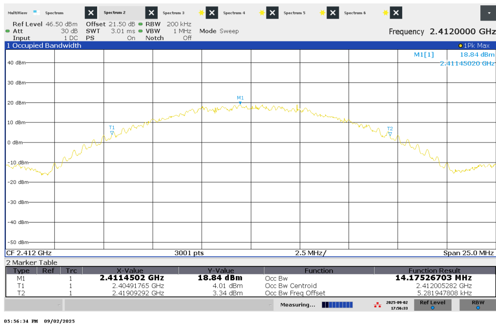
Figure 5 – 99% Bandwidth – 2412 MHz
