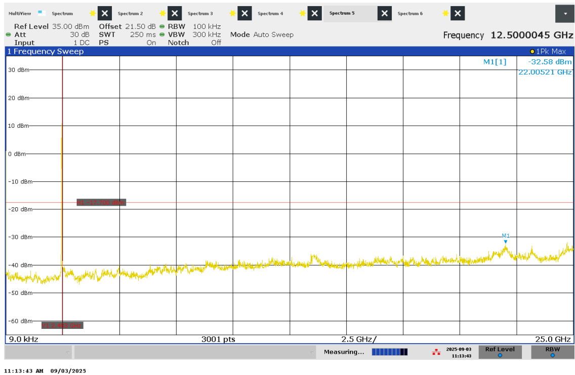
Figure 65 – -30dBc High Channel 9kHz – 25 GHz
