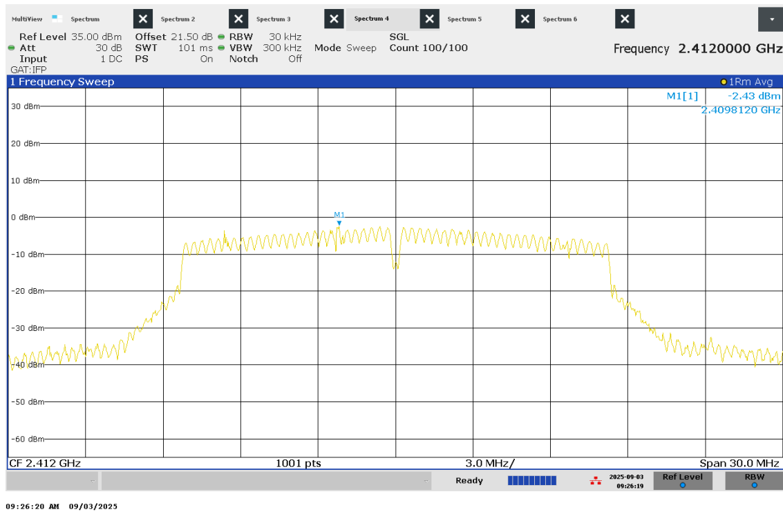
Figure 44 – PSD – Channel 1
