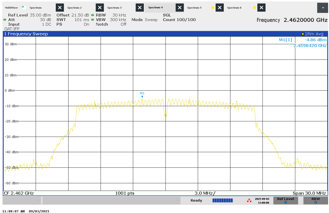
Figure 48 – PSD – Channel 11
