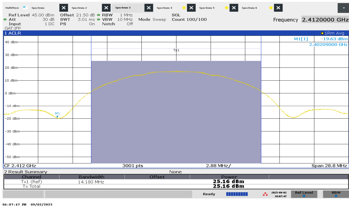
Figure 26 – Average Power - Low Channel
