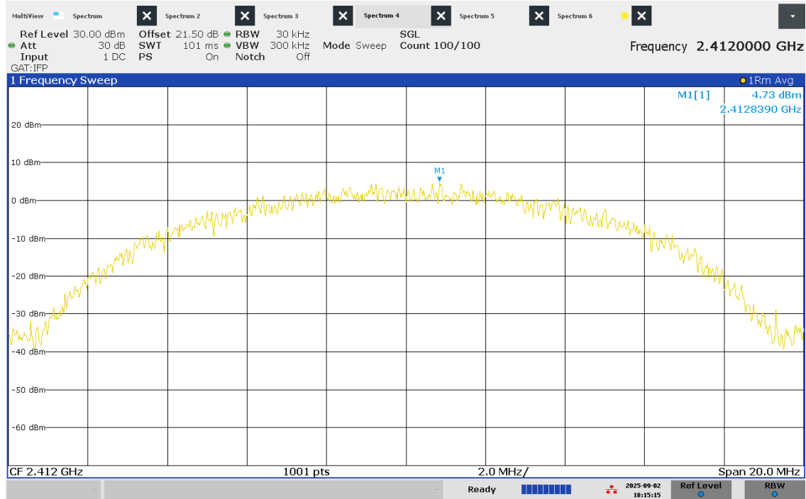
Figure 41 – PSD - Low Channel
