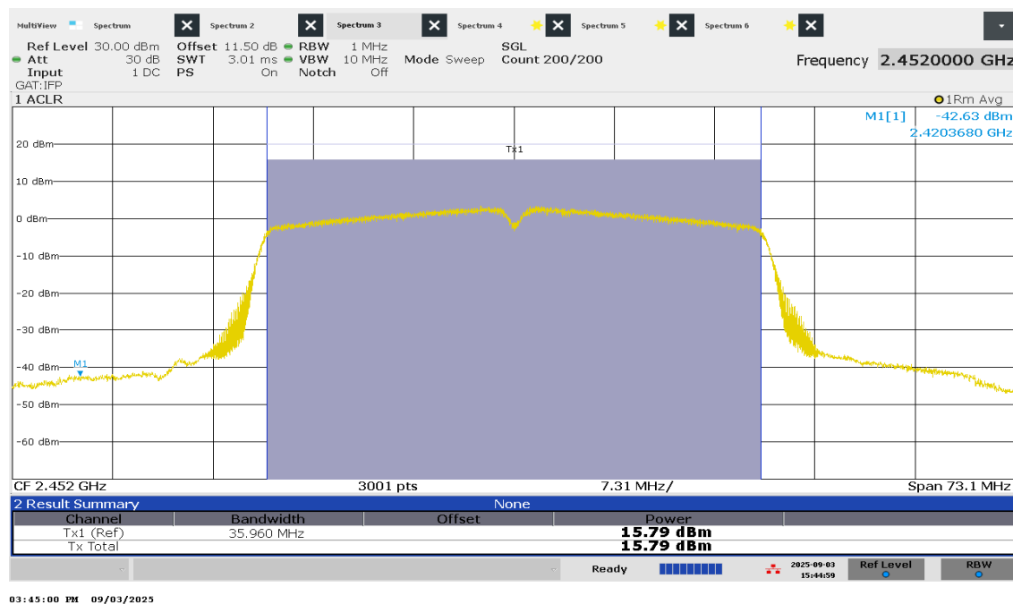
Figure 40 – Average Power - High Channel
