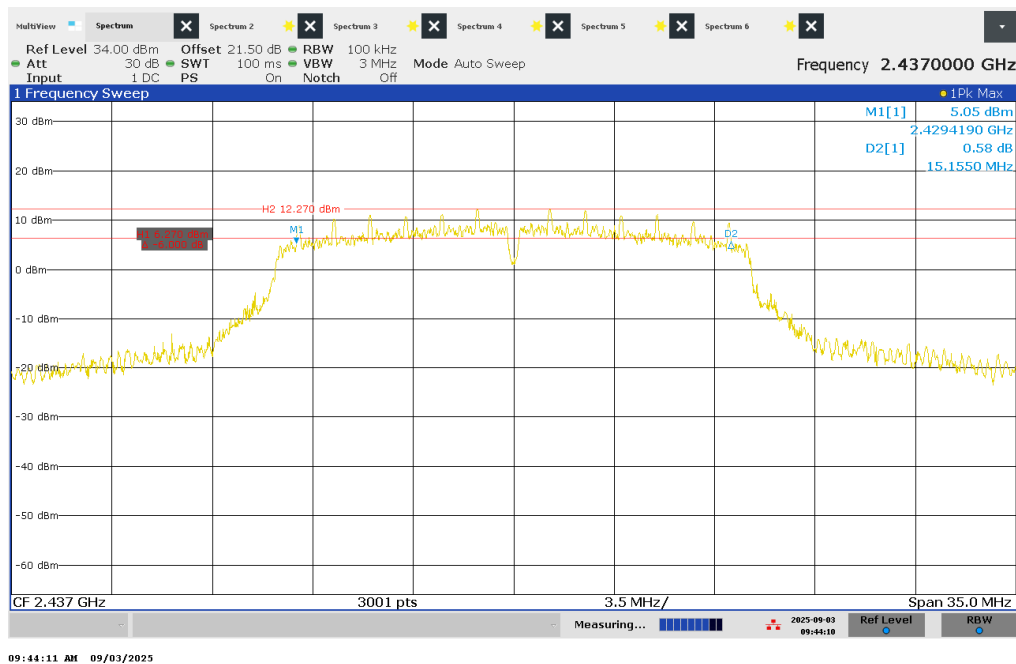
Figure 9 – 6dB Bandwidth – 2437 MHz
