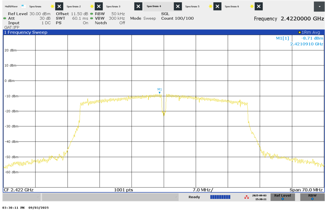
Figure 53 – PSD - Low Channel
