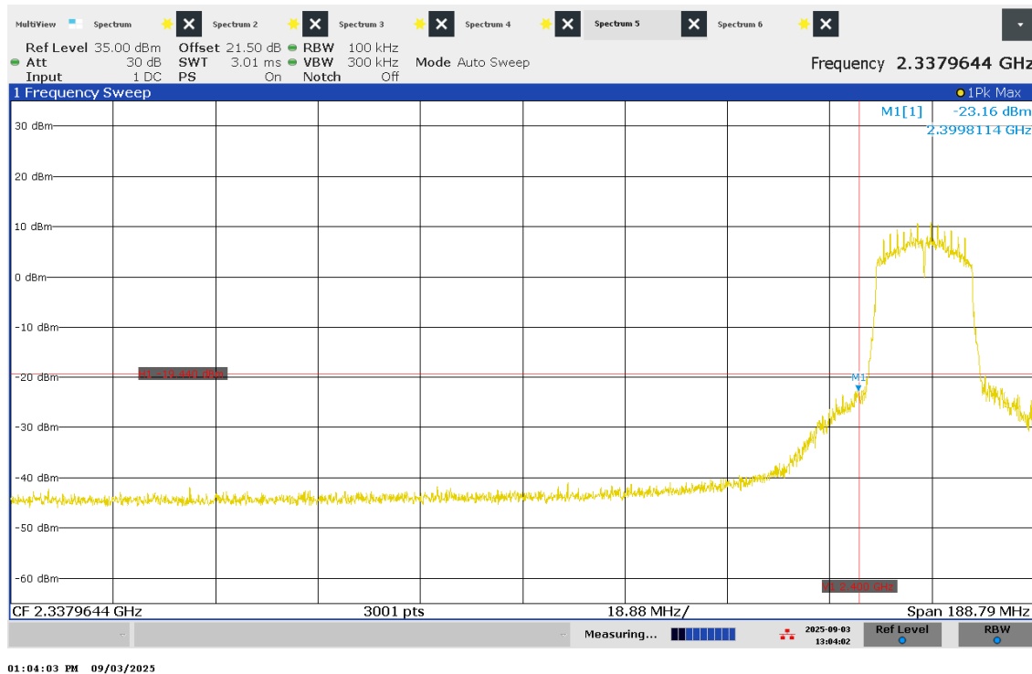
Figure 67 – -30dBc Band Edge - Low Channel
