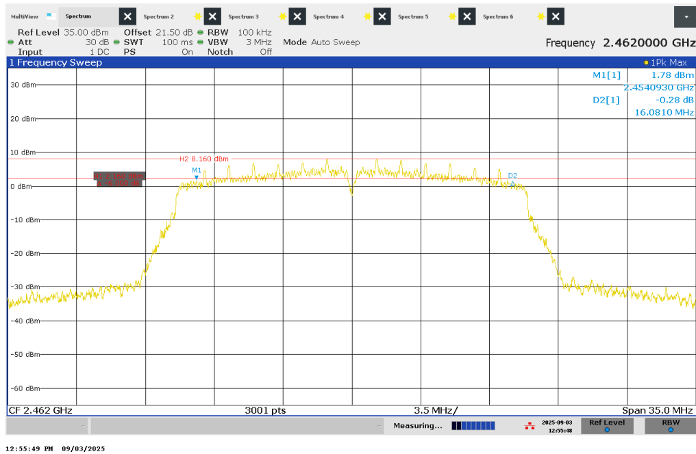
Figure 16 – 6dB Bandwidth – 2462 MHz
