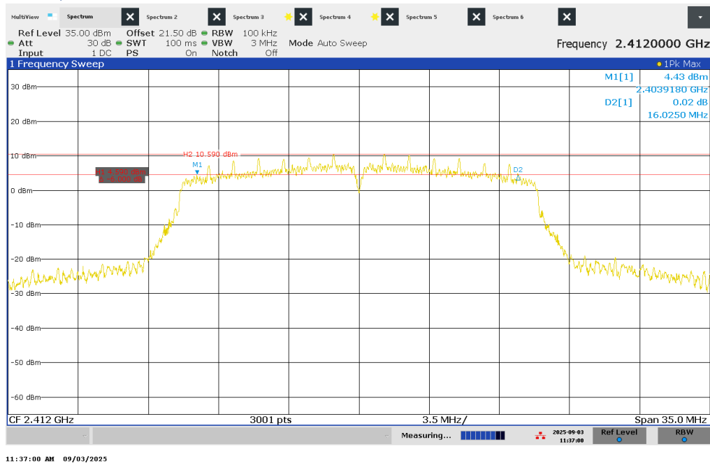
Figure 14 – 6dB Bandwidth – 2412 MHz
