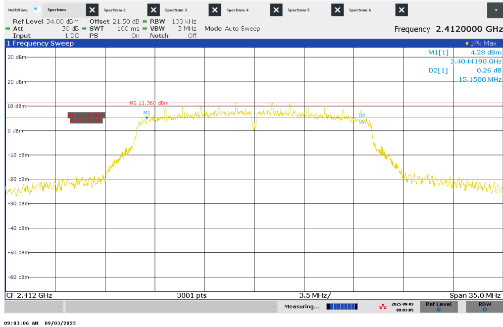
Figure 8 – 6dB Bandwidth – 2412 MHz
