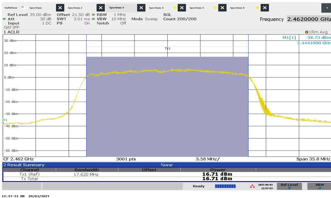
Figure 37 – Average Power - Channel 11
