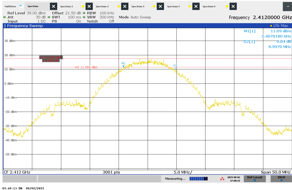
Figure 2 – 6dB Bandwidth – 2412 MHz
