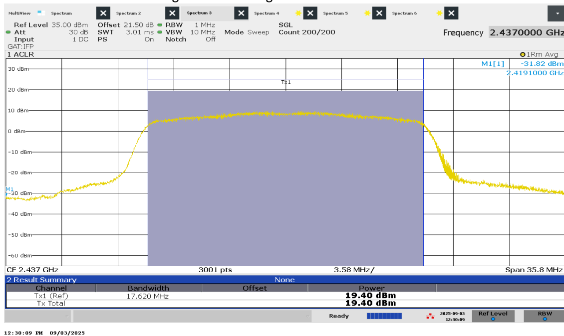
Figure 35 – Average Power - Mid Channel
