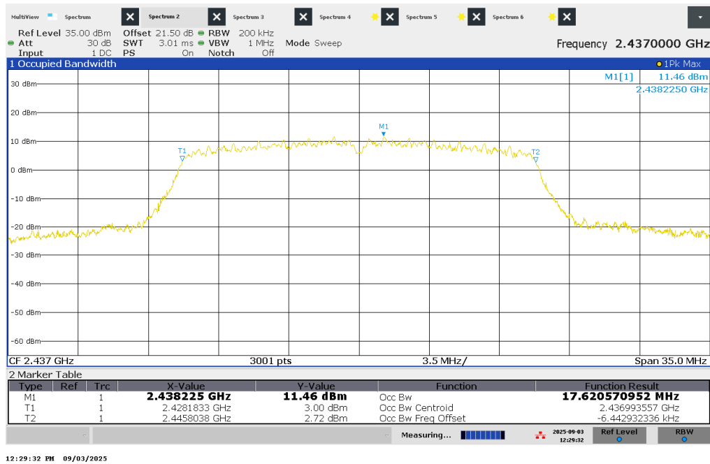
Figure 18 – 99% Bandwidth – 2437 MHz
