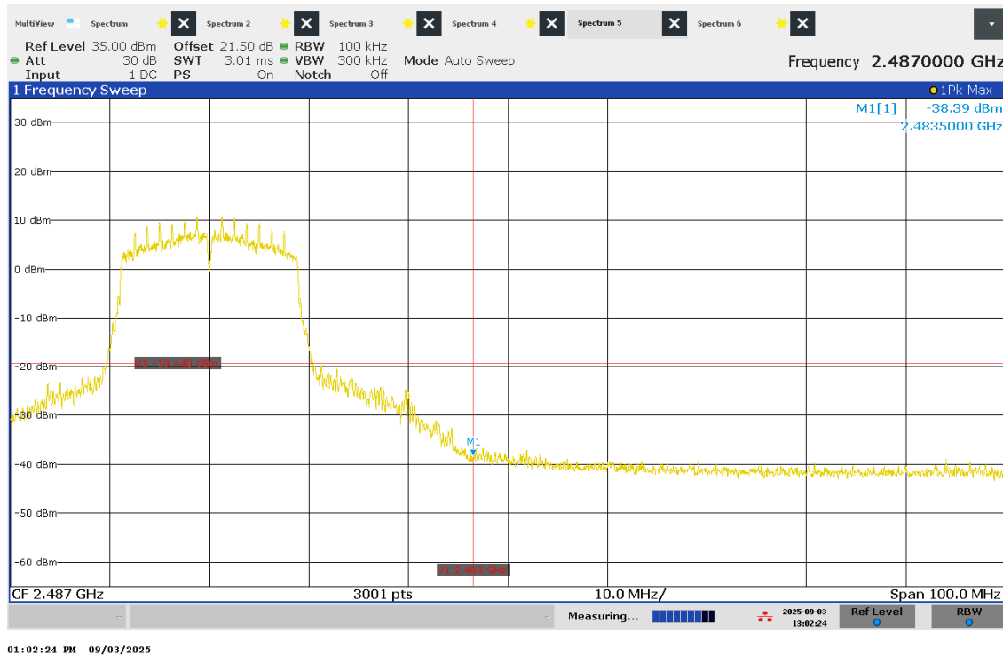
Figure 68 – -30dBc Band Edge – Channel 10
