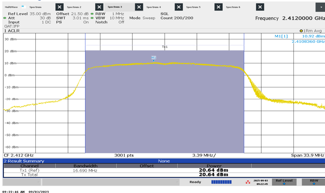
Figure 29 – Average Power – Channel 1
