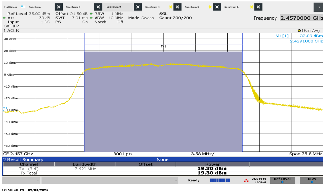
Figure 36 – Average Power - Channel 10
