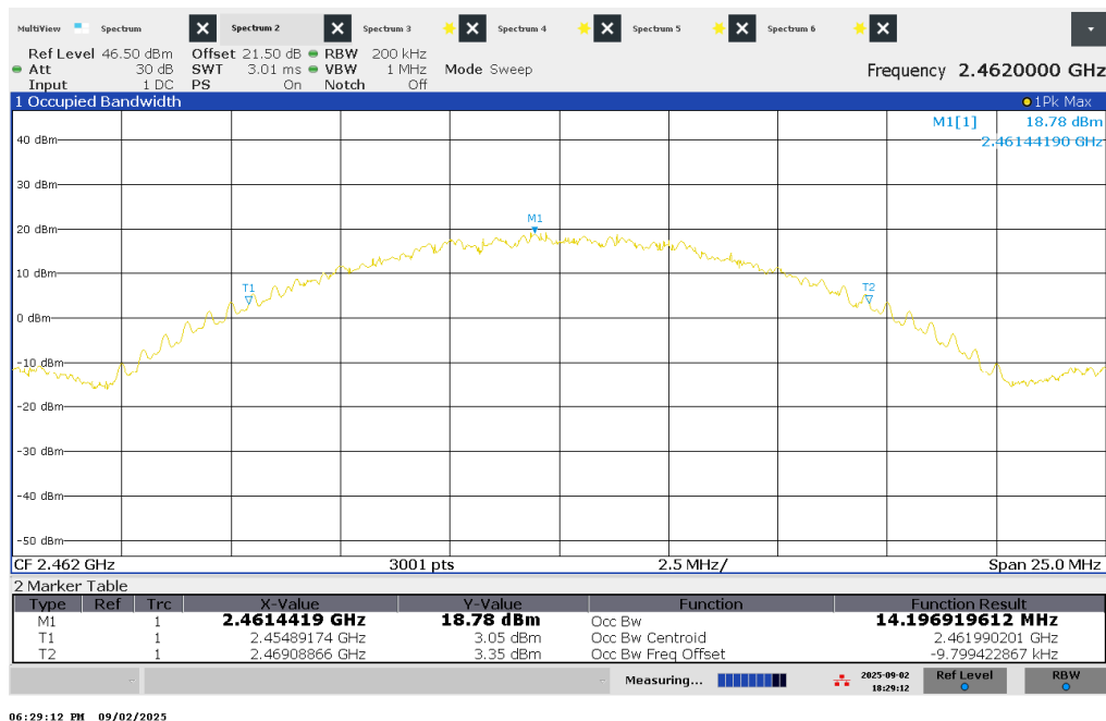
Figure 7 – 99% Bandwidth – 2462 MHz
