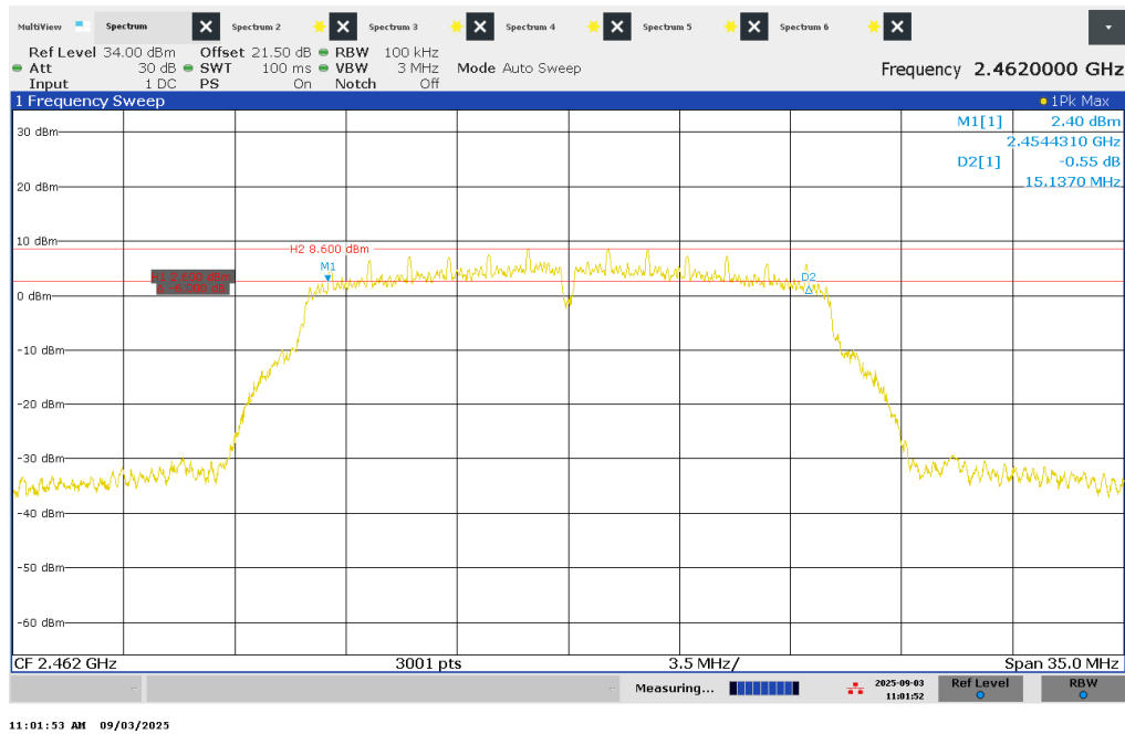
Figure 10 – 6dB Bandwidth – 2462 MHz
