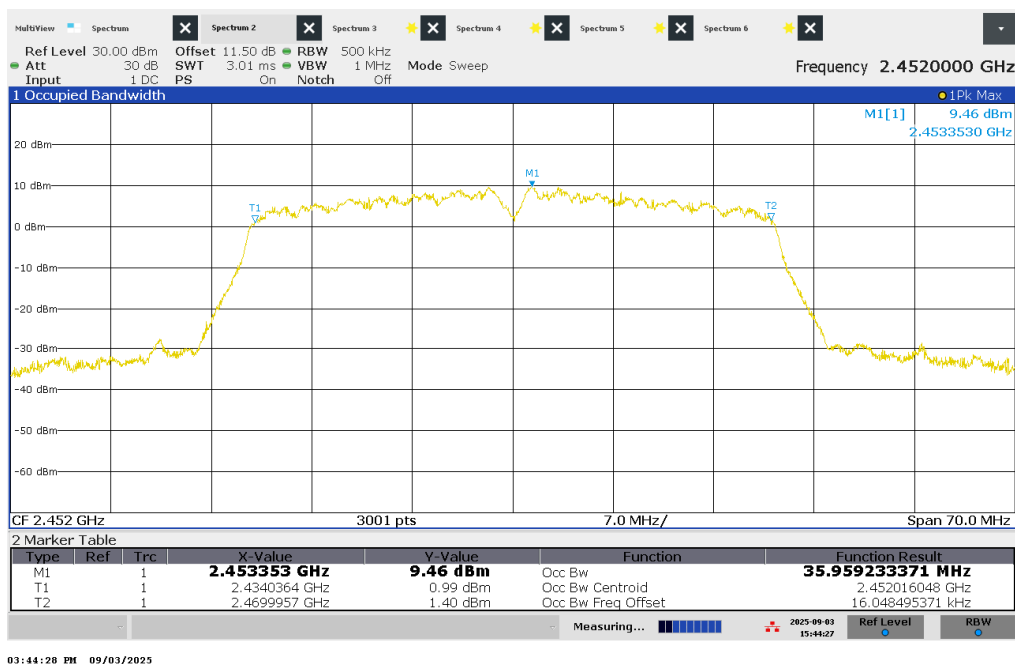
Figure 25 – 99% Bandwidth – 2452 MHz
