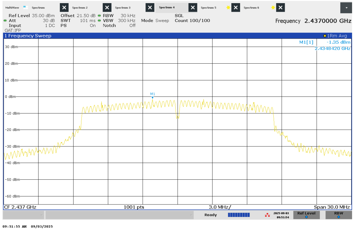
Figure 46 – PSD - Mid Channel
