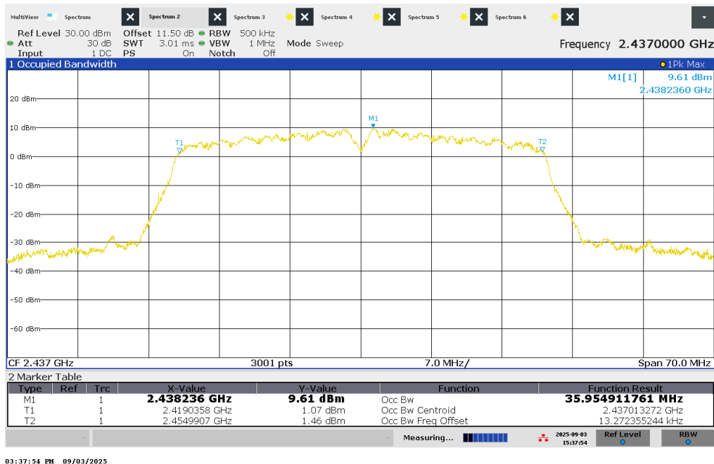
Figure 24 – 99% Bandwidth – 2437 MHz
