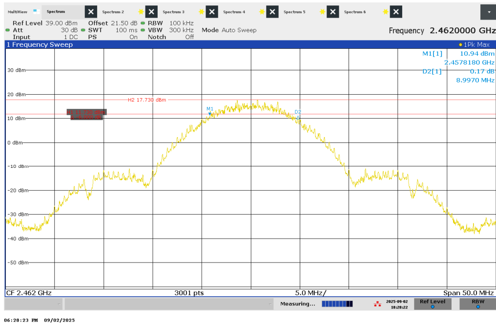
Figure 4 – 6dB Bandwidth – 2462 MHz
