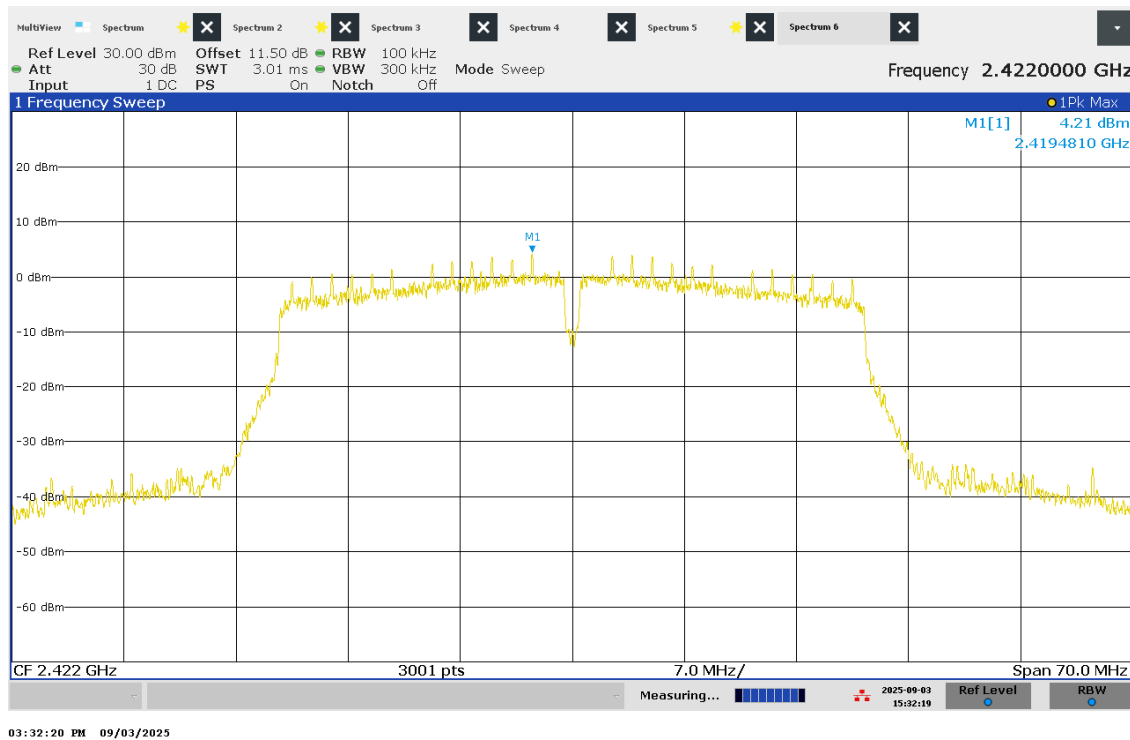
Figure 71 – -30dBc Reference Level
