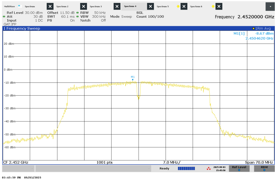
Figure 55 – PSD - High Channel
