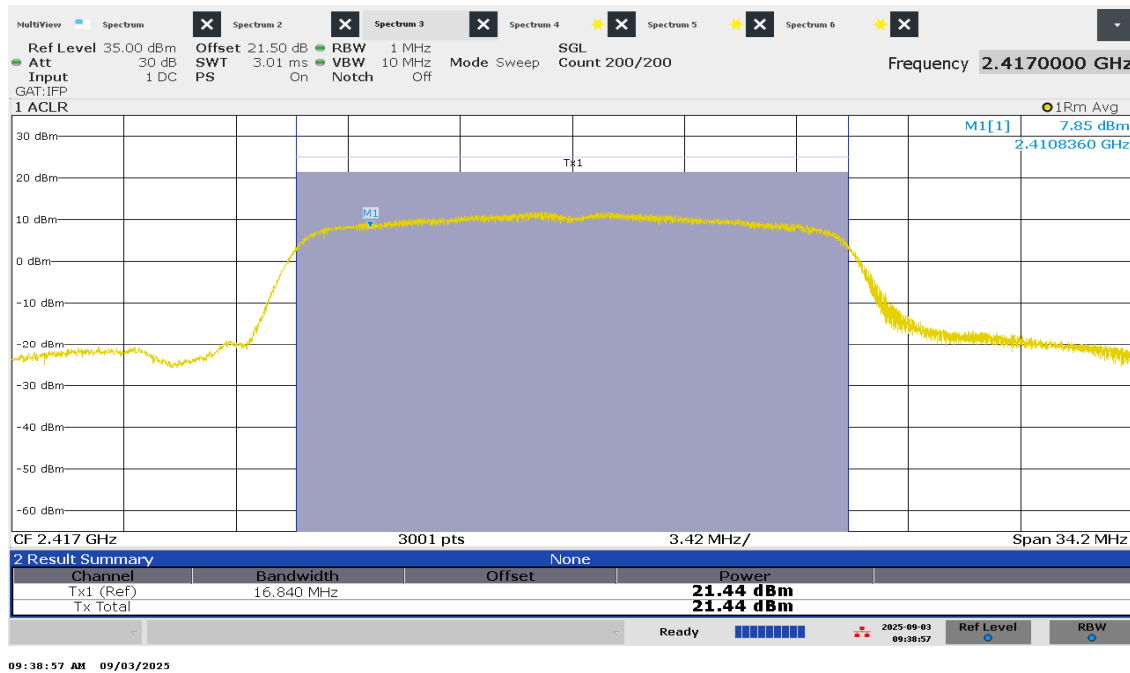
Figure 30 – Average Power – Channel 2
