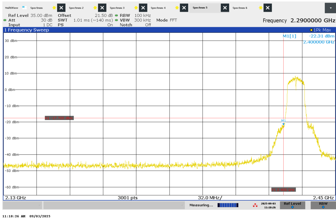
Figure 61 – -30dBc Band Edge – Channel 1
