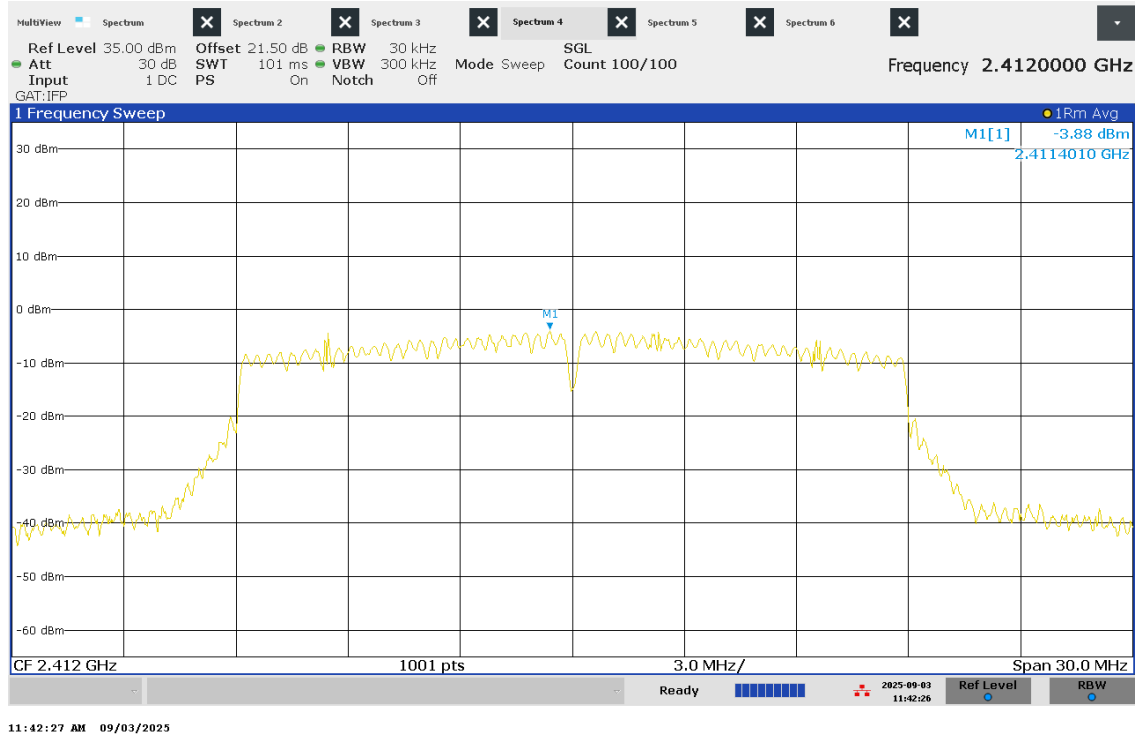
Figure 49 – PSD - Low Channel
