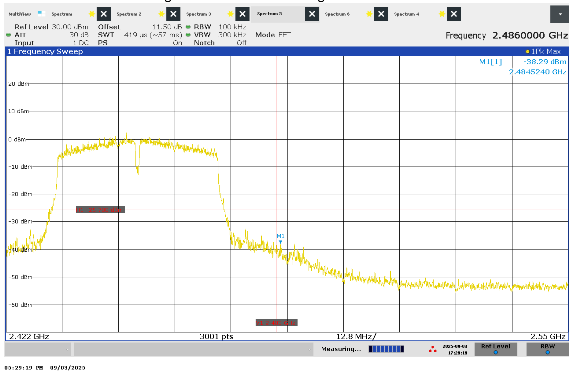
Figure 73 – -30dBc Band Edge - High Channel
