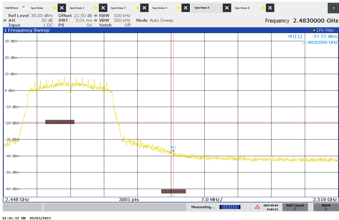
Figure 69 – -30dBc Band Edge – Channel 11
