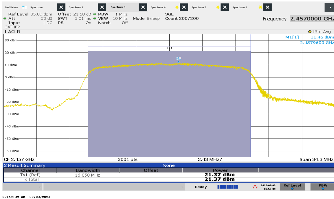
Figure 32 – Average Power – Channel 10
