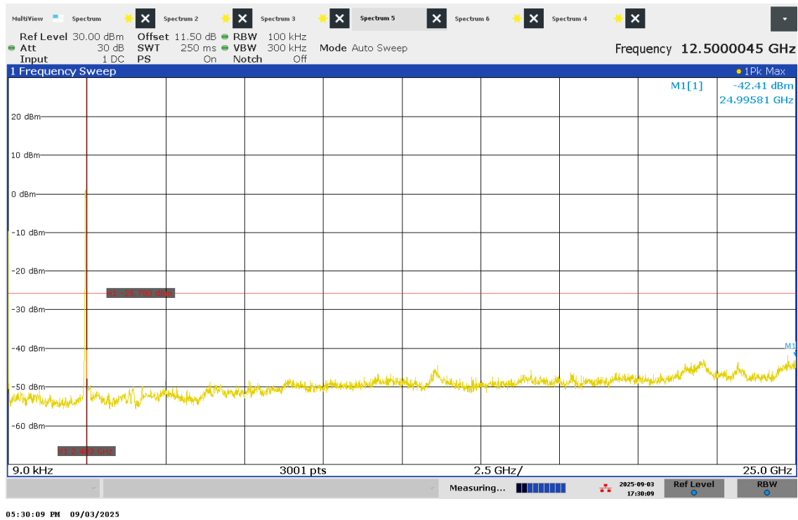
Figure 74 – -30dBc High Channel 9kHz – 25 GHz
