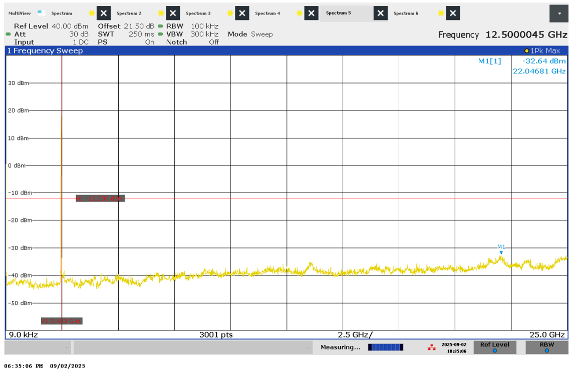
Figure 59 – -30dBc High Channel 9kHz – 25 GHz
