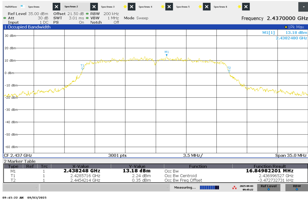
Figure 12 – 99% Bandwidth – 2437 MHz
