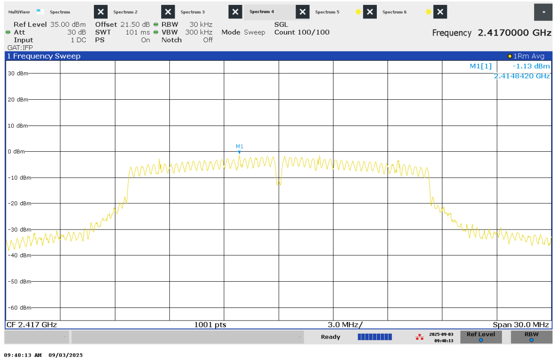
Figure 45 – PSD – Channel 2
