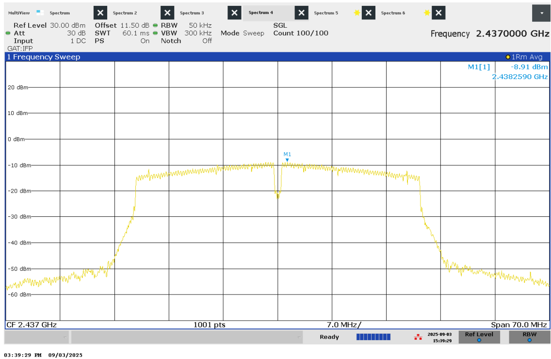
Figure 54 – PSD - Mid Channel
