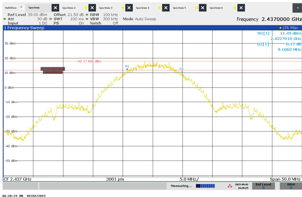
Figure 3 – 6dB Bandwidth – 2437 MHz
