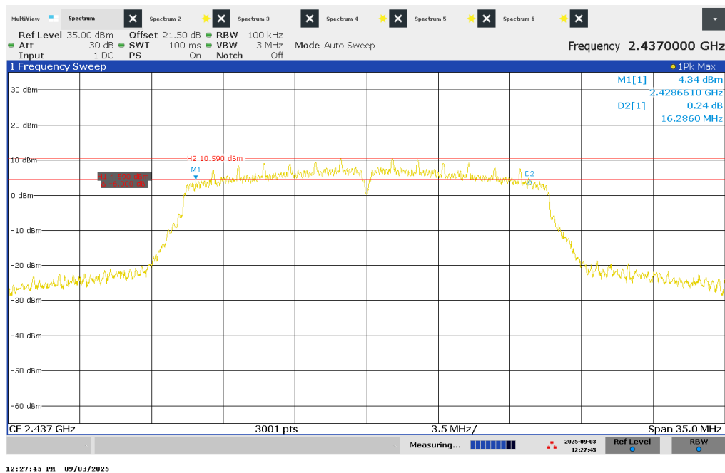
Figure 15 – 6dB Bandwidth – 2437 MHz
