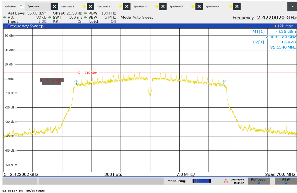
Figure 20 – 6dB Bandwidth – 2422 MHz
