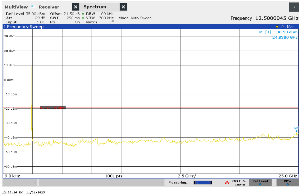
Figure 70 – -30dBc High Channel 9kHz – 25 GHz
