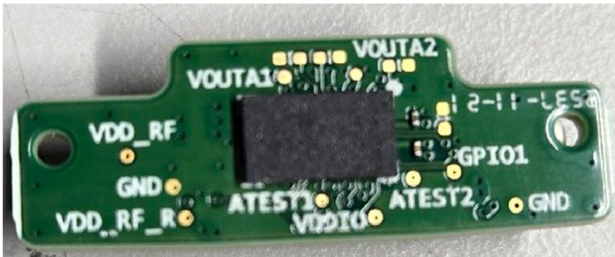
Figure 2 – Bottom view
