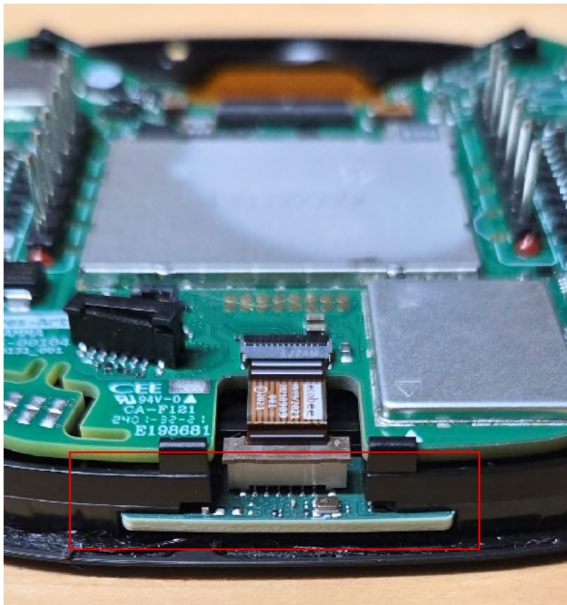
Figure 2 – Internal view (red box is location of EB-SOC60G)
