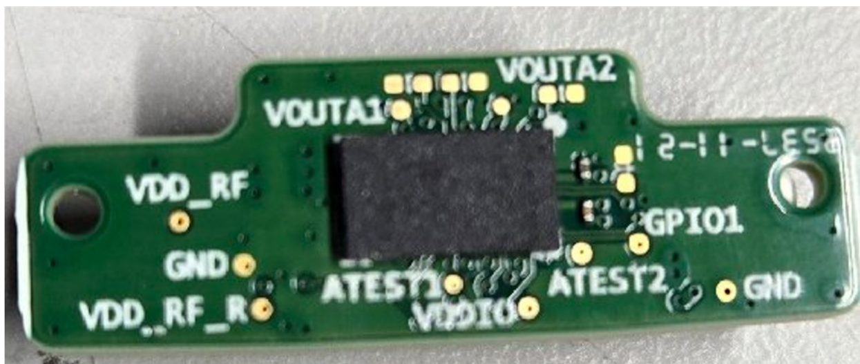
Figure 2 – Bottom view
