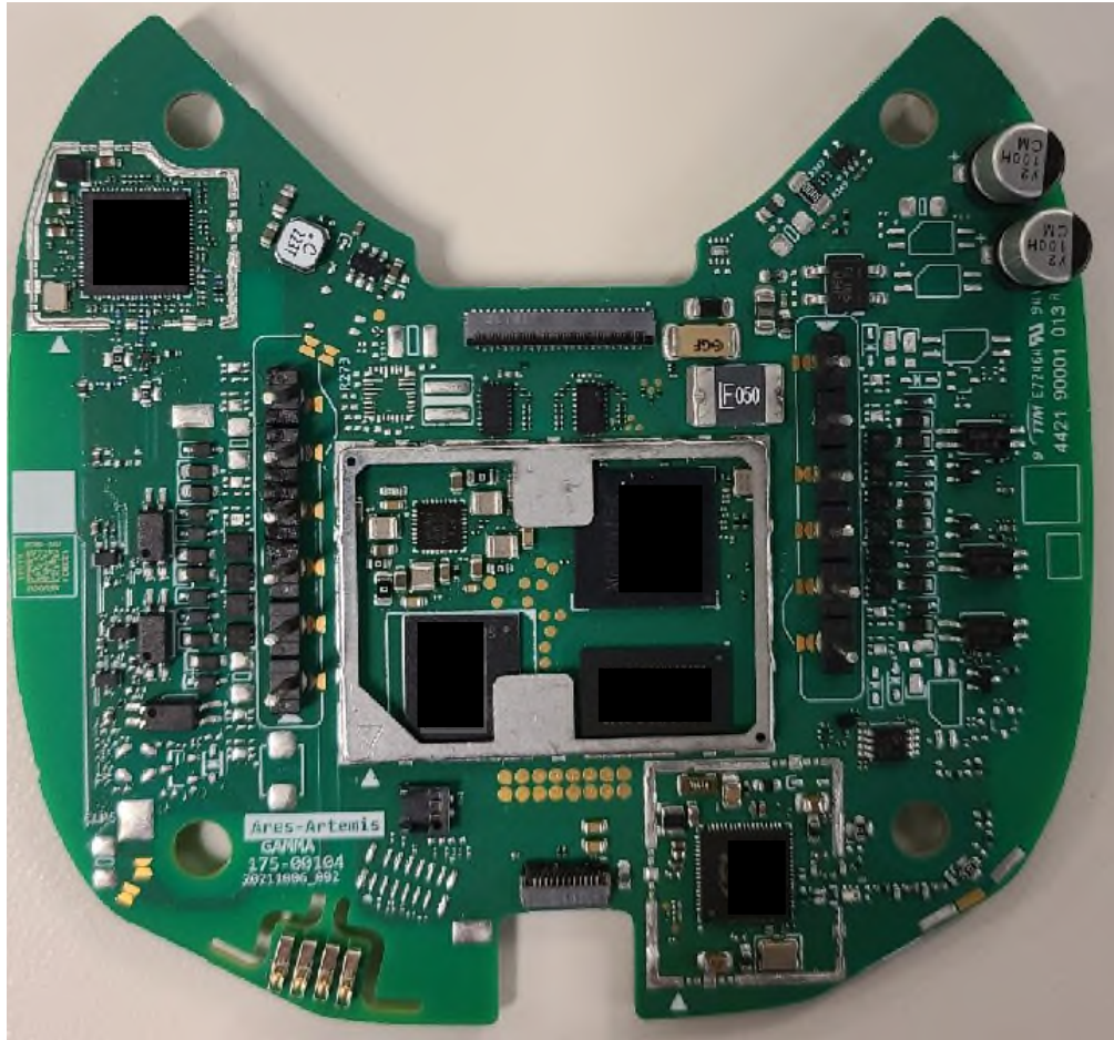
Figure 4 – ECB601 Internal Photo 3
