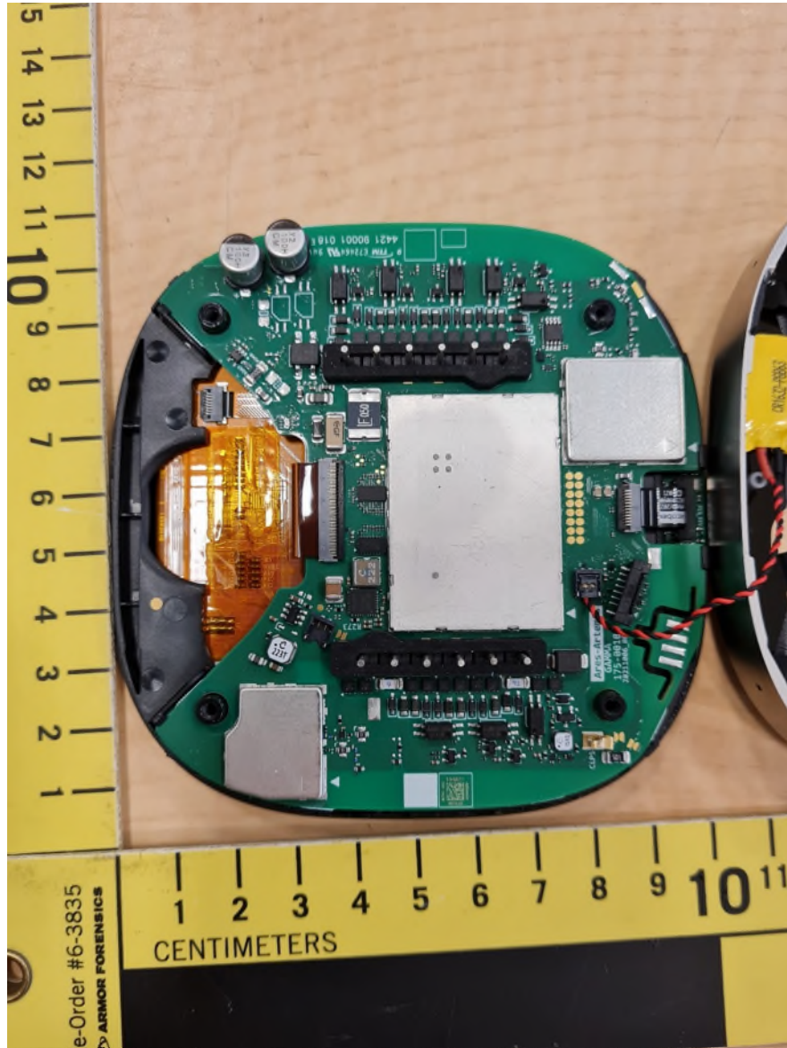
Figure 3 – ECB601 Internal Photo 3
