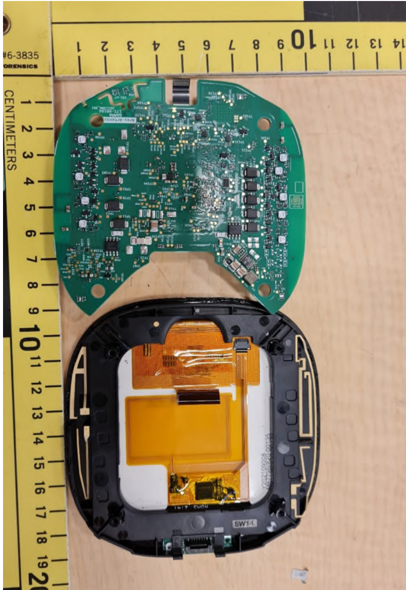
Figure 2 – ECB601 Internal Photo 2
