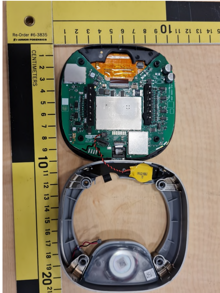
Figure 1 – ECB601 Internal Photo 1t
