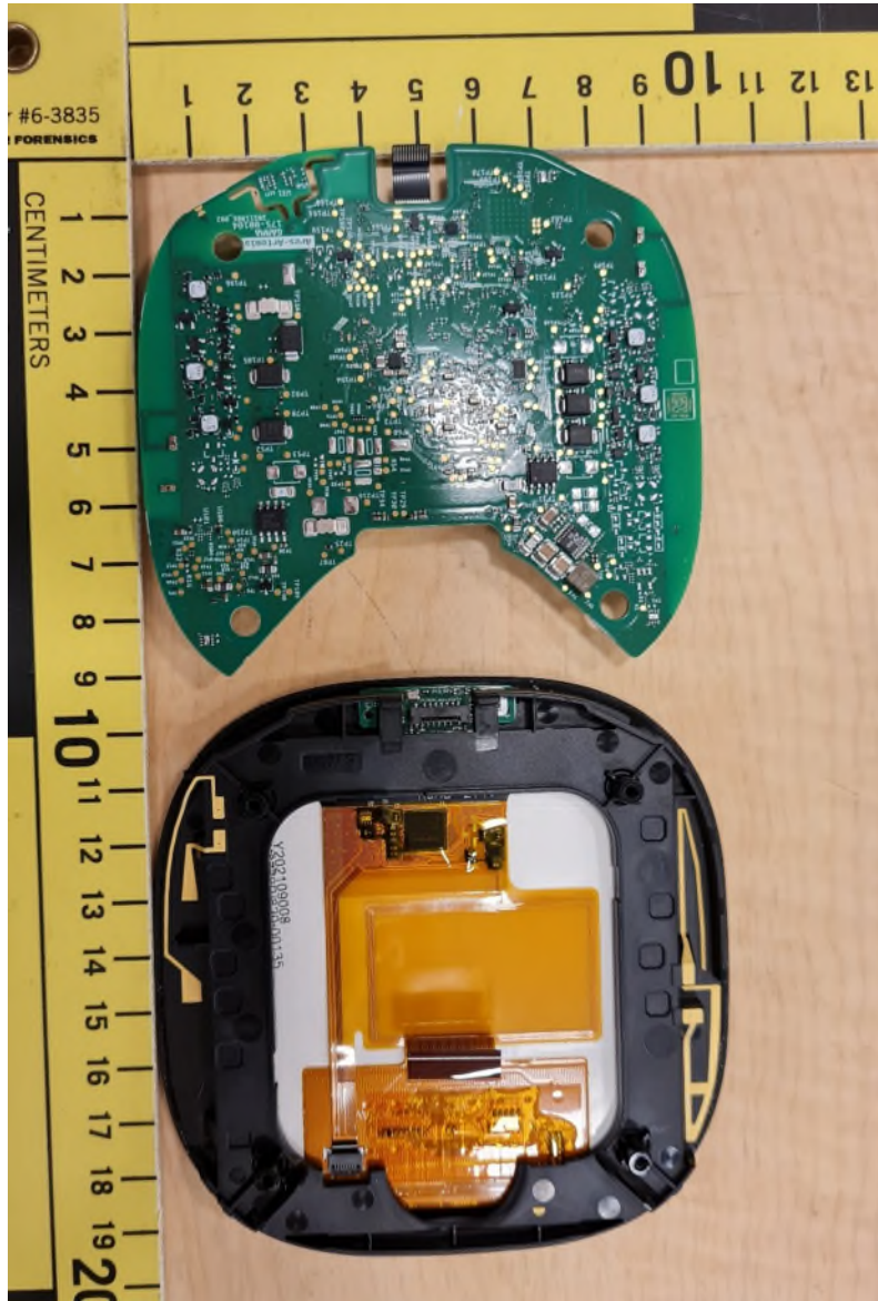
Figure 6 – ECB501 Internal Photo 2
