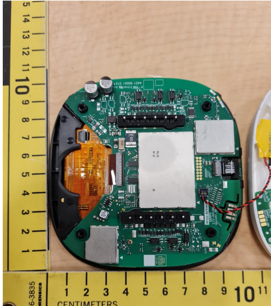
Figure 7 – ECB501 Internal Photo 3
