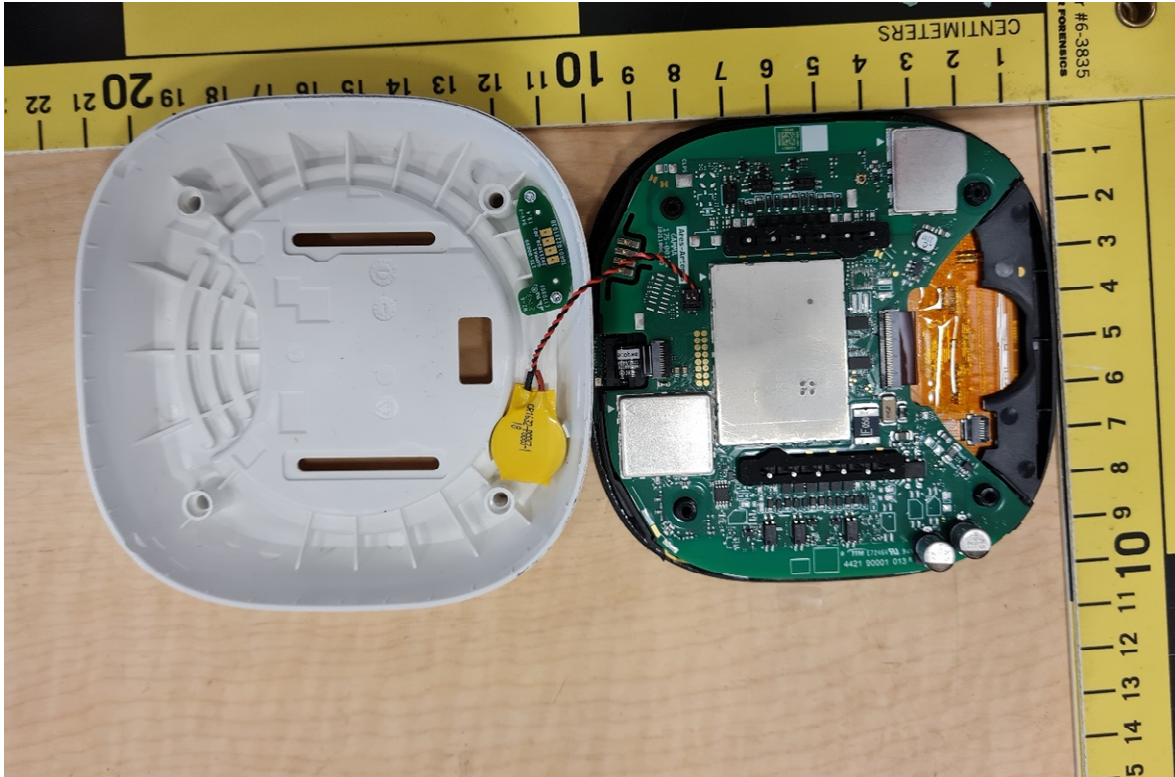
Figure 5 – ECB501 Internal Photo 1t
