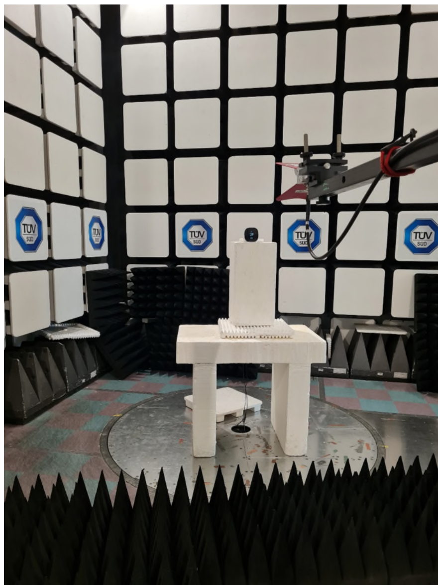
Figure 4 – Radiated Emissions Setup 1 > 1GHz
