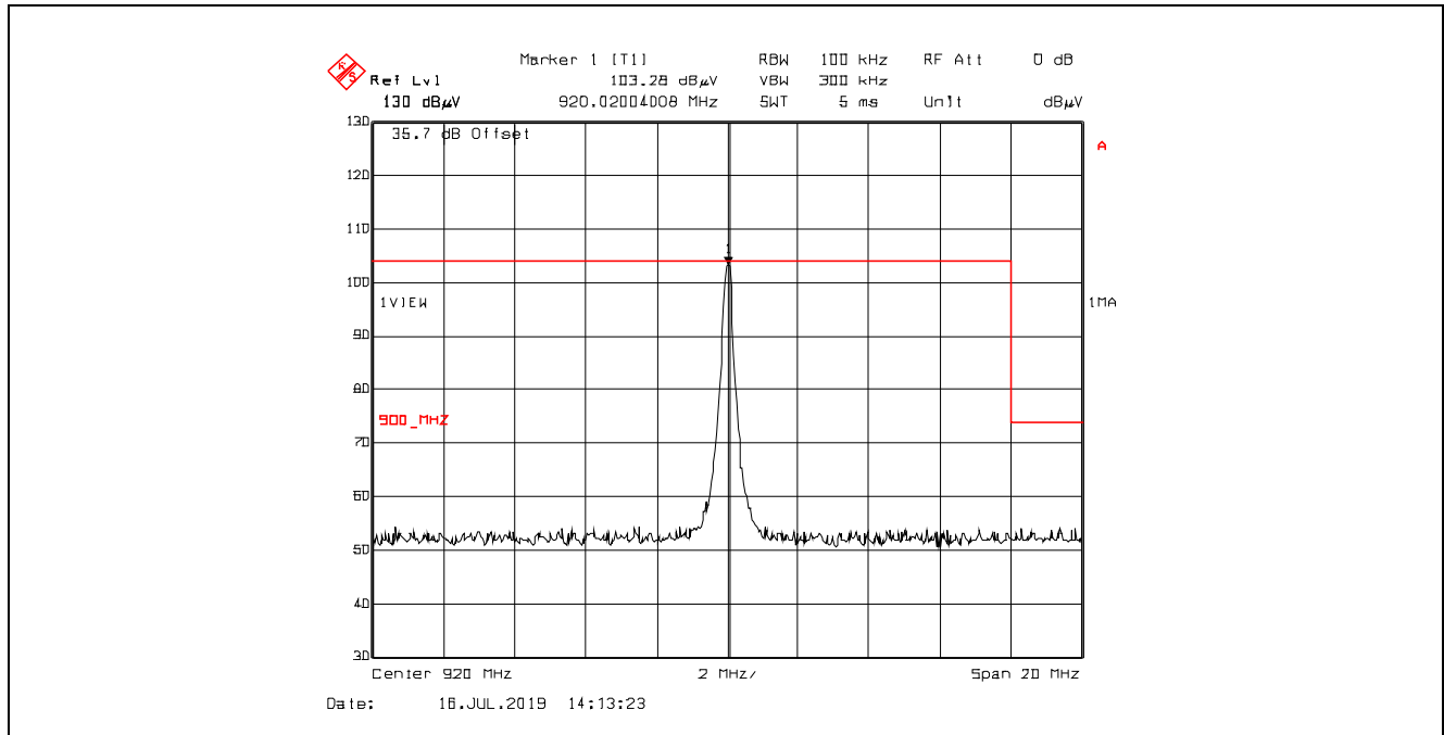
Plot 5.5.4.2.1. Band-Edge RF Radiated Emissions at 3 m, Horizontal Polarization Single Frequency Mode, 920.00 MHz
