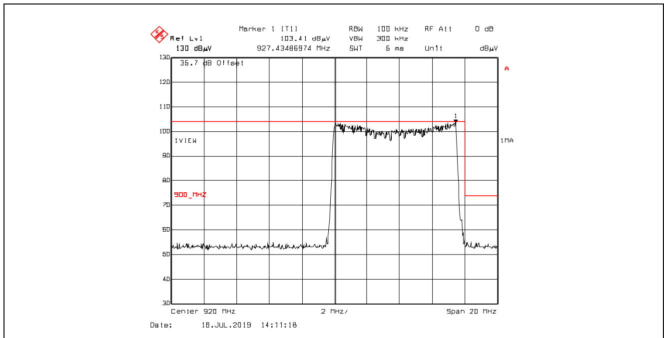
Plot 5.5.4.2.2. Band-Edge RF Radiated Emissions at 3 m, Horizontal Polarization Pseudorandom Channel Hopping Mode, 920.00 MHz
