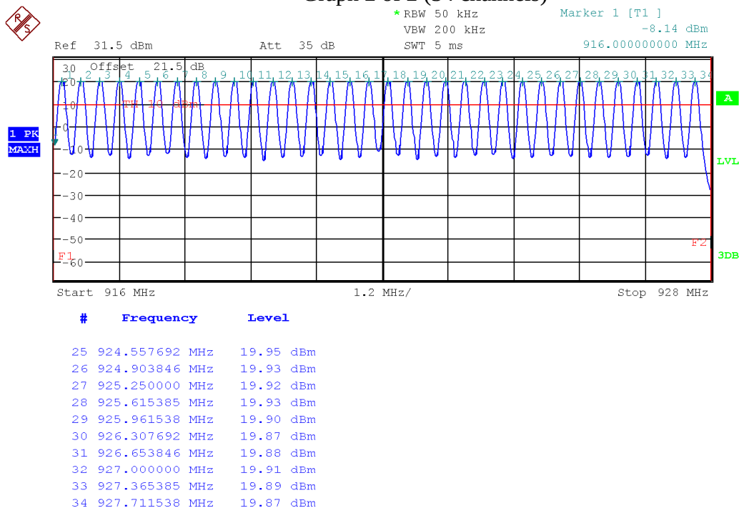
Graph 2 of 2 (34 channels)
