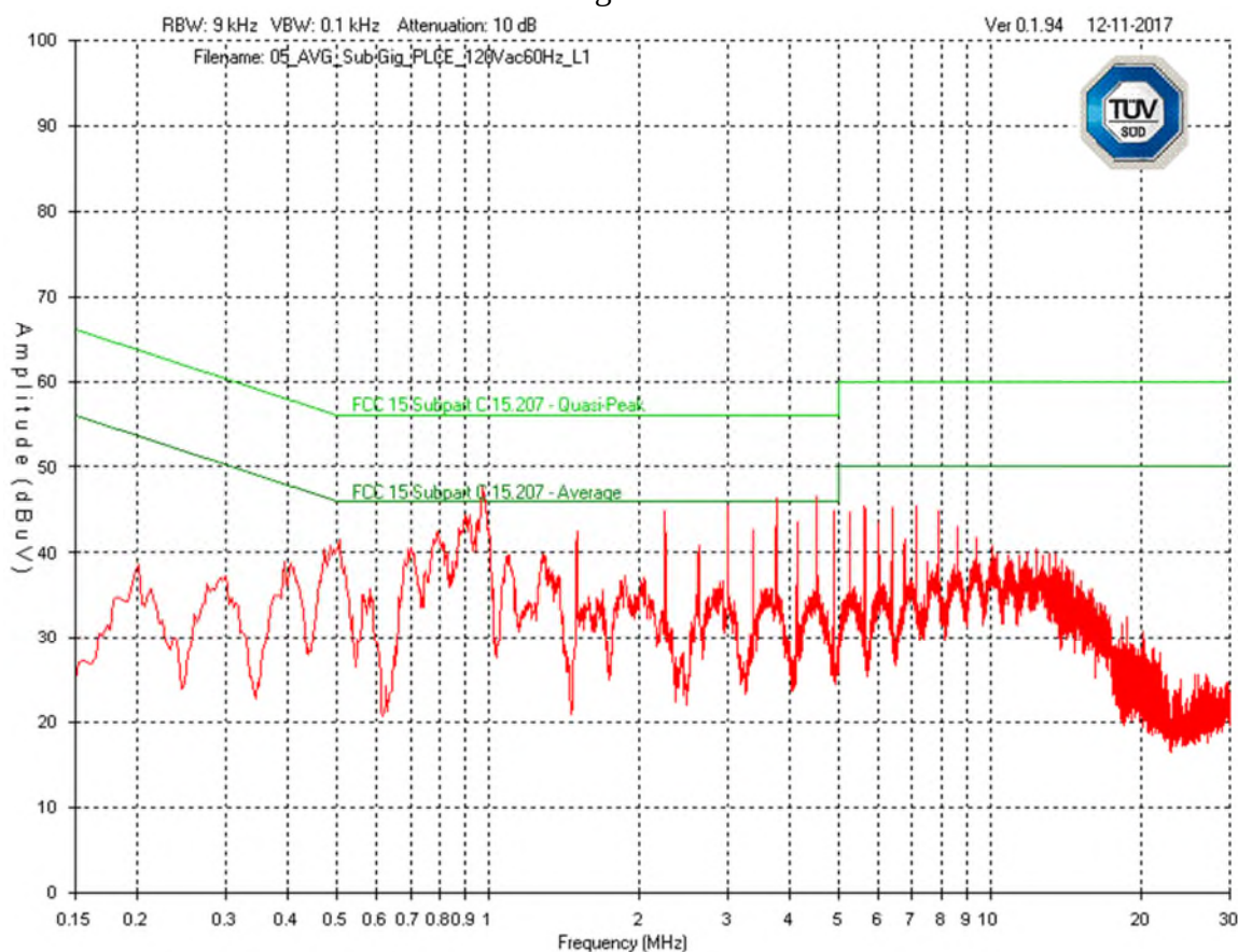
Line (L1) – 120Vac 60Hz Average Emission
