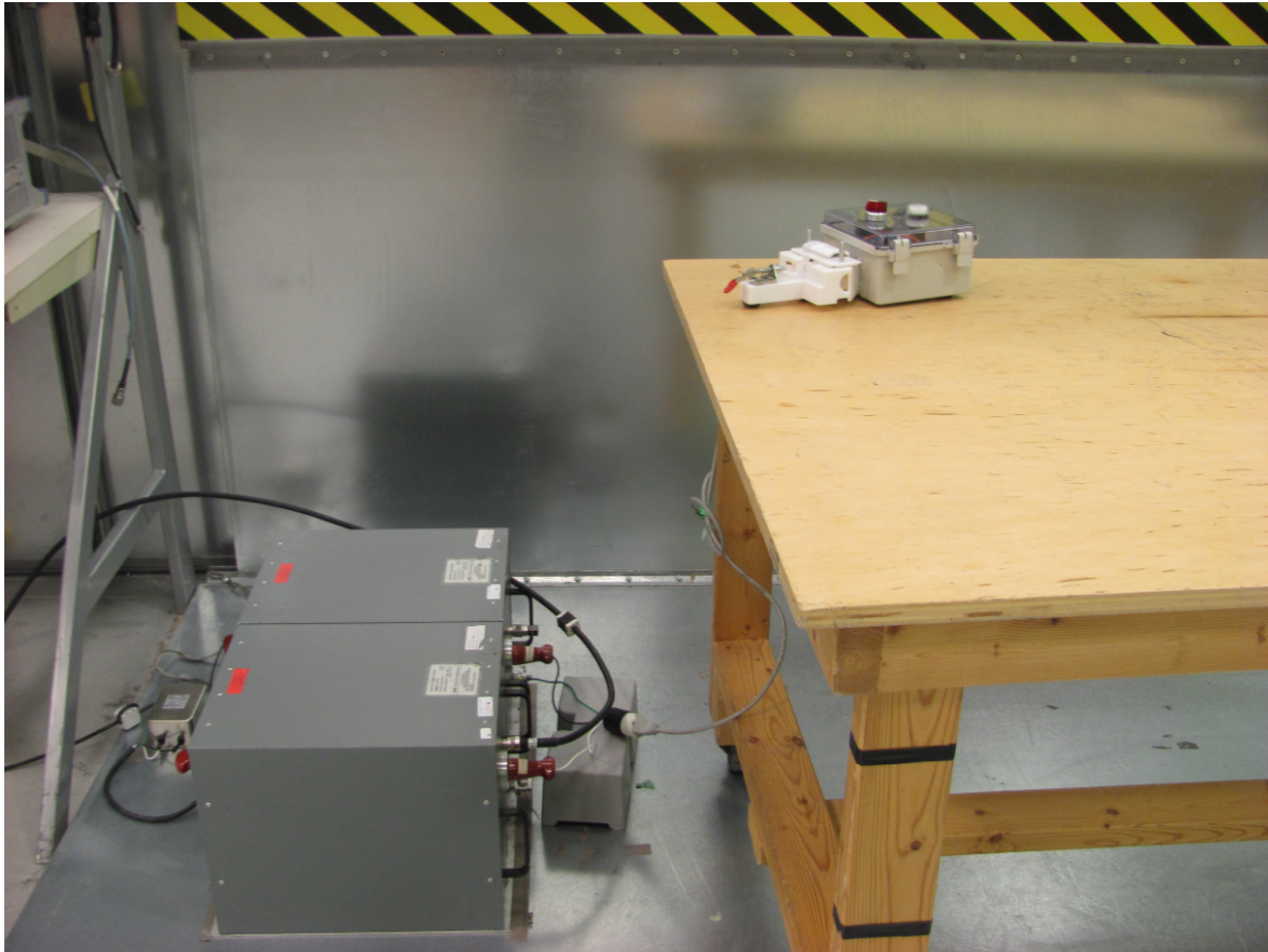
Figure 7 – Power Line Conducted Emissions Setup – Photo 1
