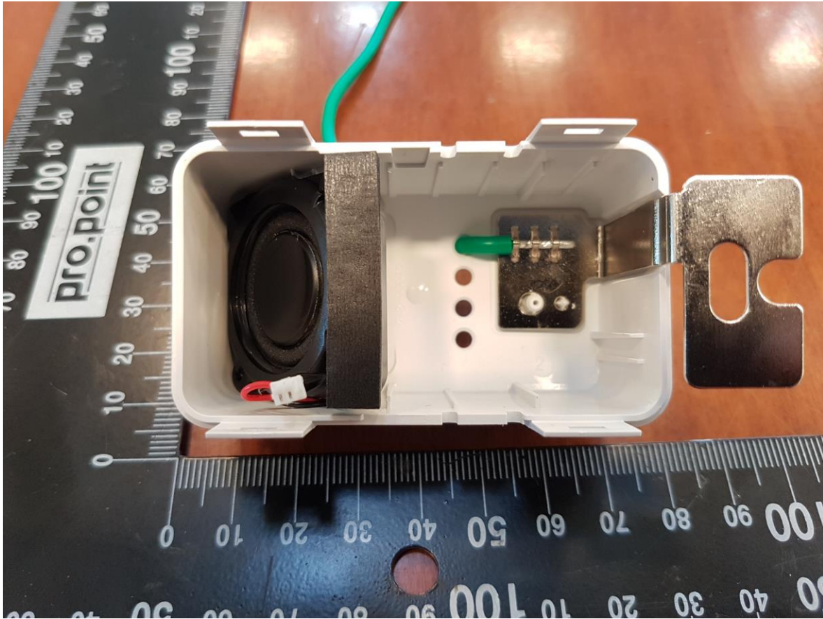
Figure 2 – EUT Internal View – photo 2
