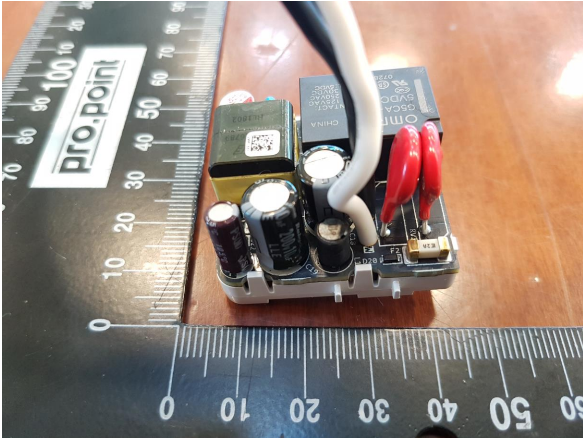
Figure 4 – EUT Internal View, PSU side – Photo 2
