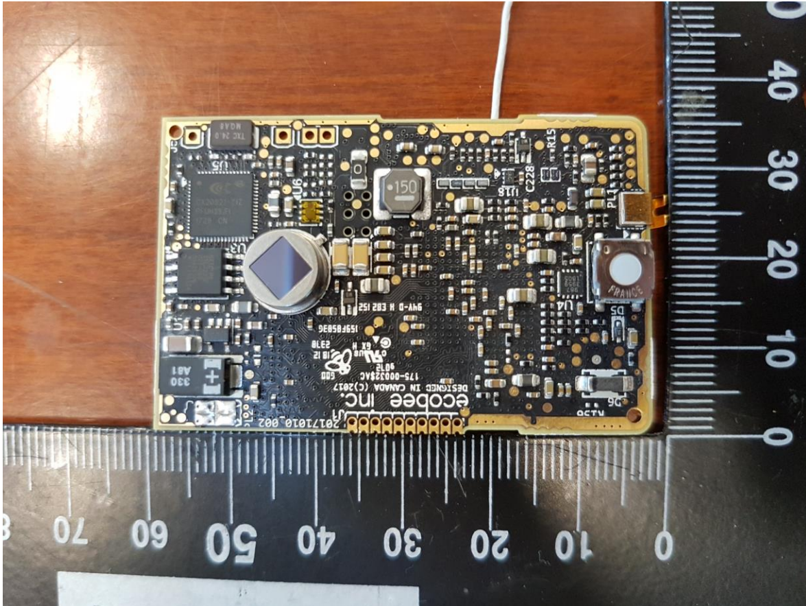
Figure 5 – EUT Internal View, Main Board – Photo 1
