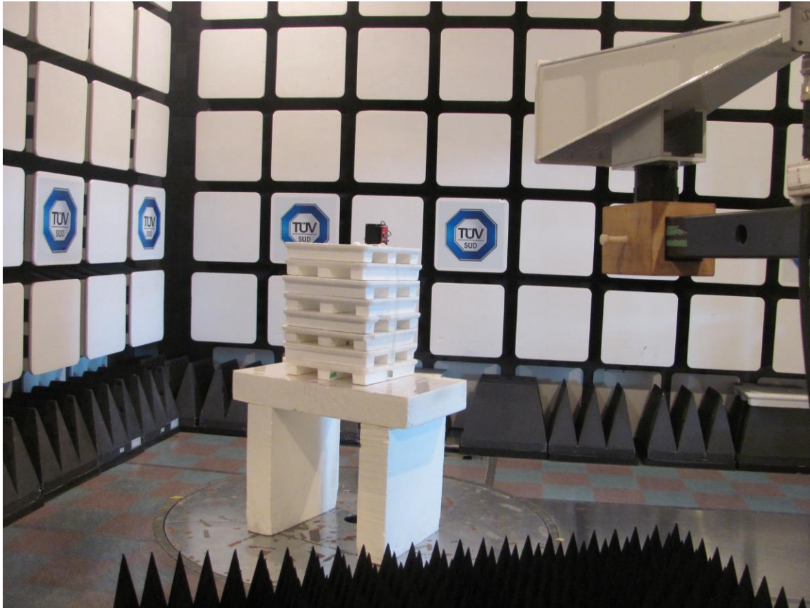
Figure 5 – Radiated Emissions Setup – Photo 4
