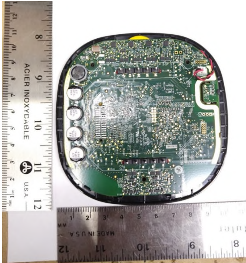
Figure 2 – EUT Internal View, PCB Back – photo 2
