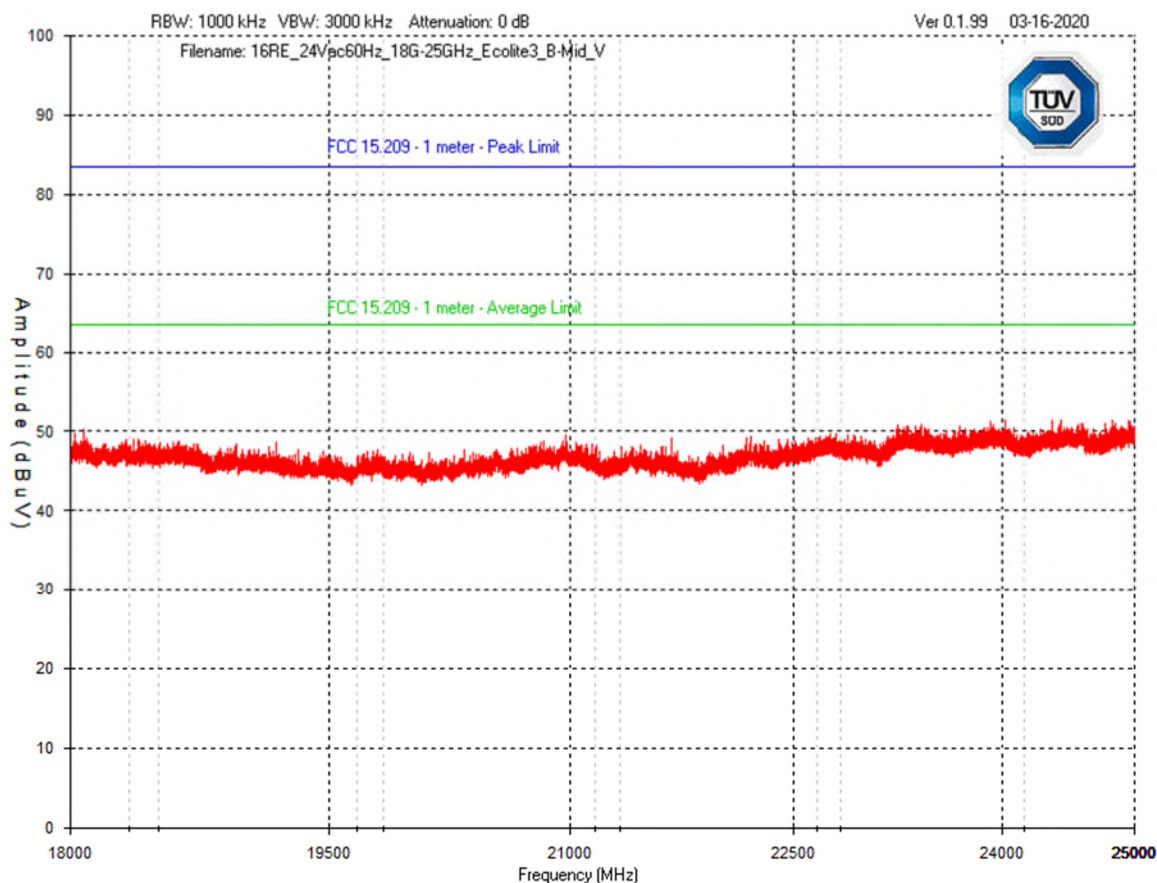
B-Mode, Mid Channel – 18 GHz – 25 GHz Vertical - Peak Emission Graph
