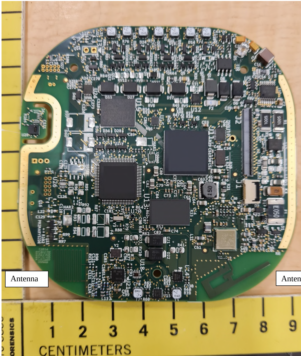
Figure 3 – EUT Internal Photo 3
