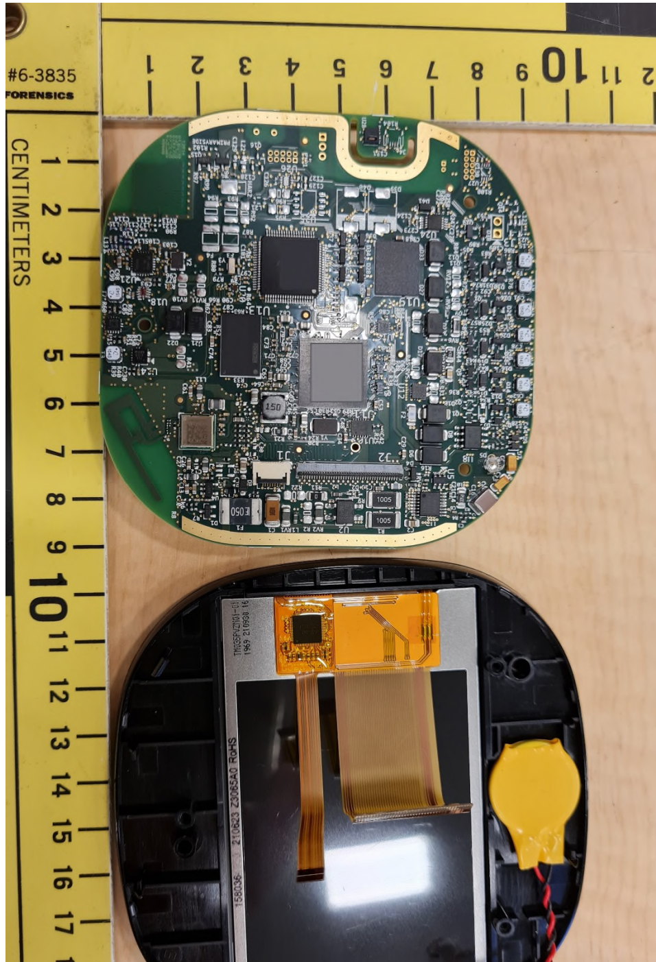
Figure 2 – EUT Internal Photo 2
