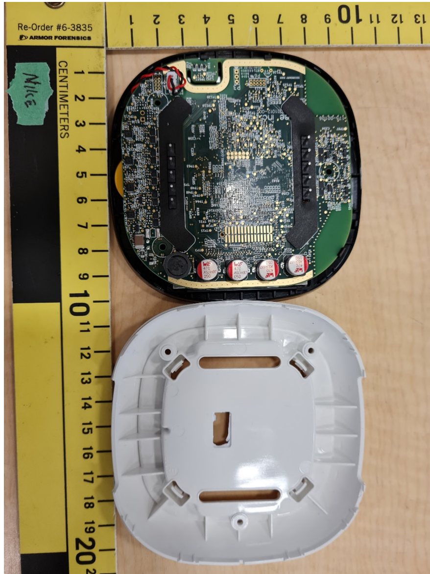
Figure 1 – EUT Internal Photo 1t
