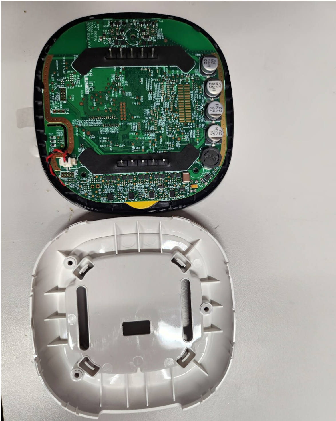
Figure 1 – EUT Internal Photo 1t
