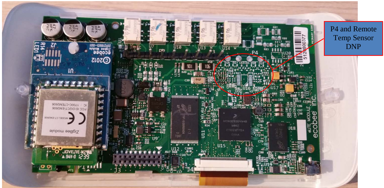
Illustration 2: EUT internal view with modularly certified Zigbee module – photo 1
