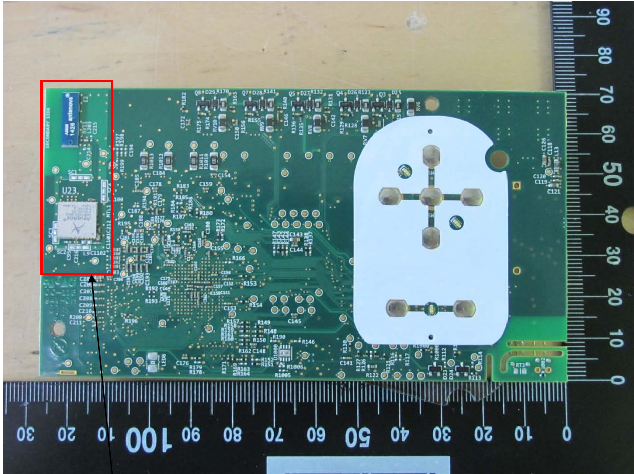
Illustration 5: EUT internal view – photo 4
