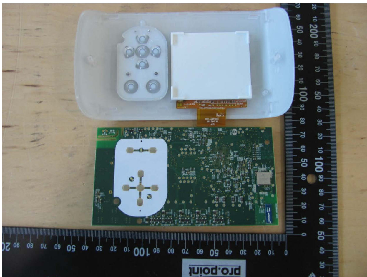
Illustration 4: EUT internal view – photo 3
