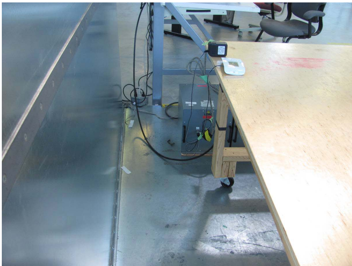
Figure 8: Power line conducted emission setup – photo 2
