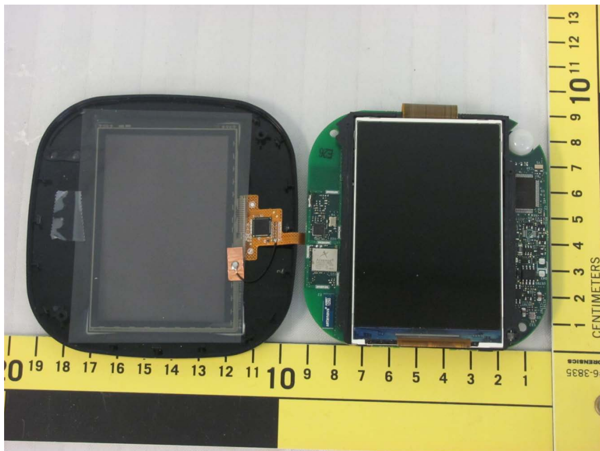
Illustration 3: EUT internal front view – photo
