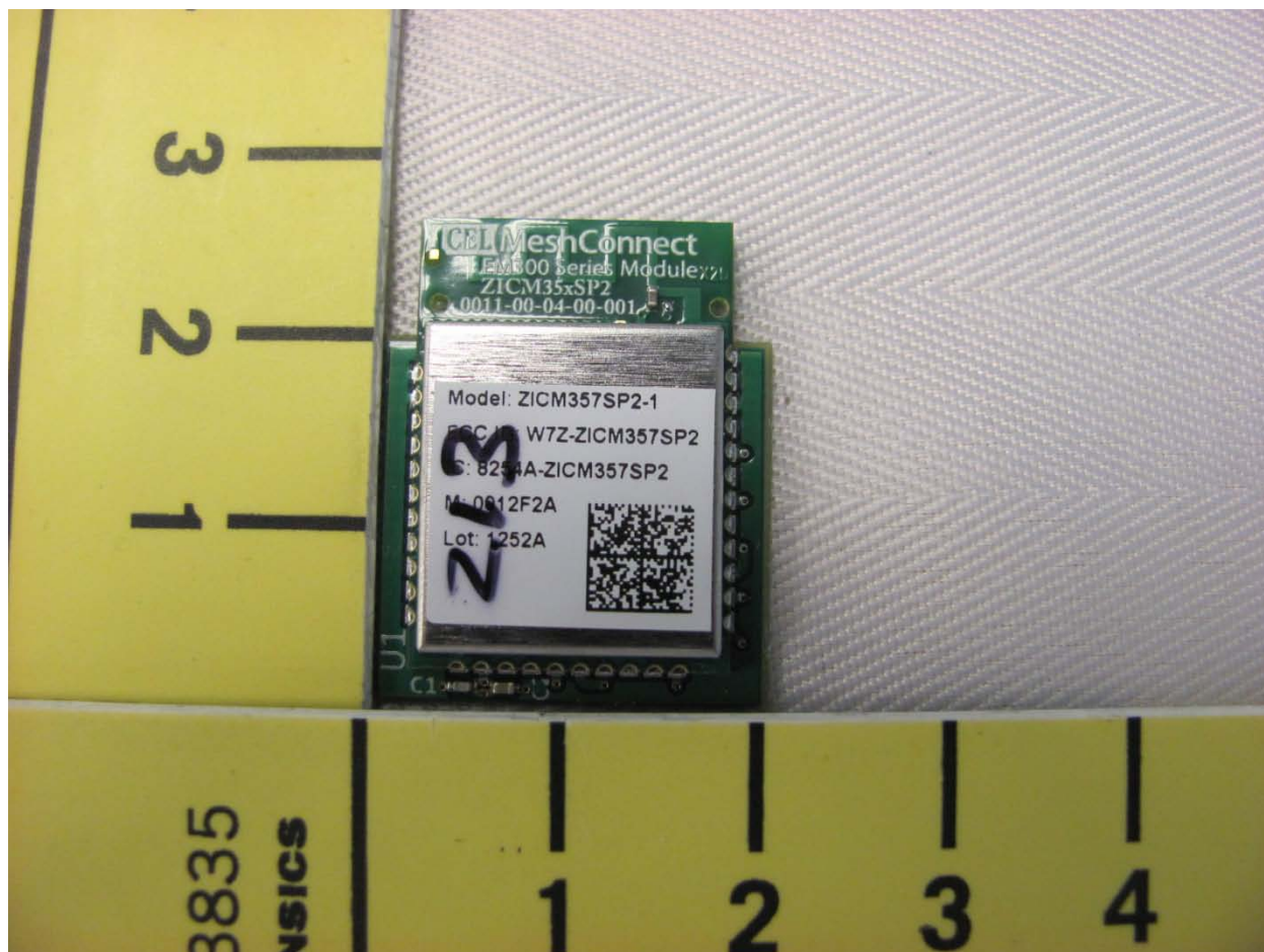
Illustration 2: Zigbee module
