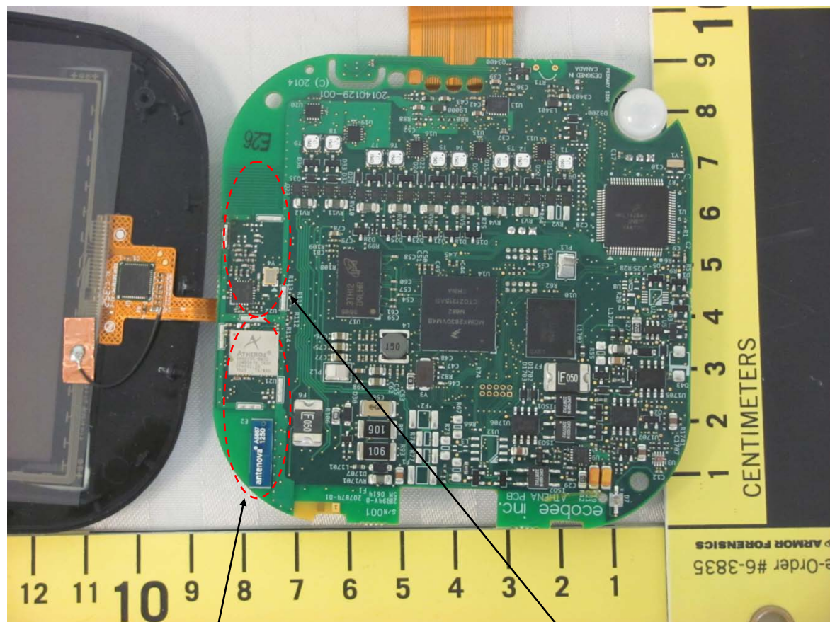
Illustration 4: EUT internal view – photo
