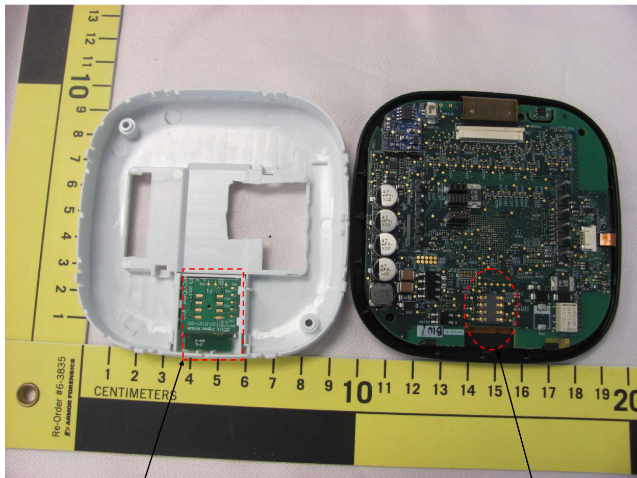
Illustration 1: EUT internal rear view – photo
