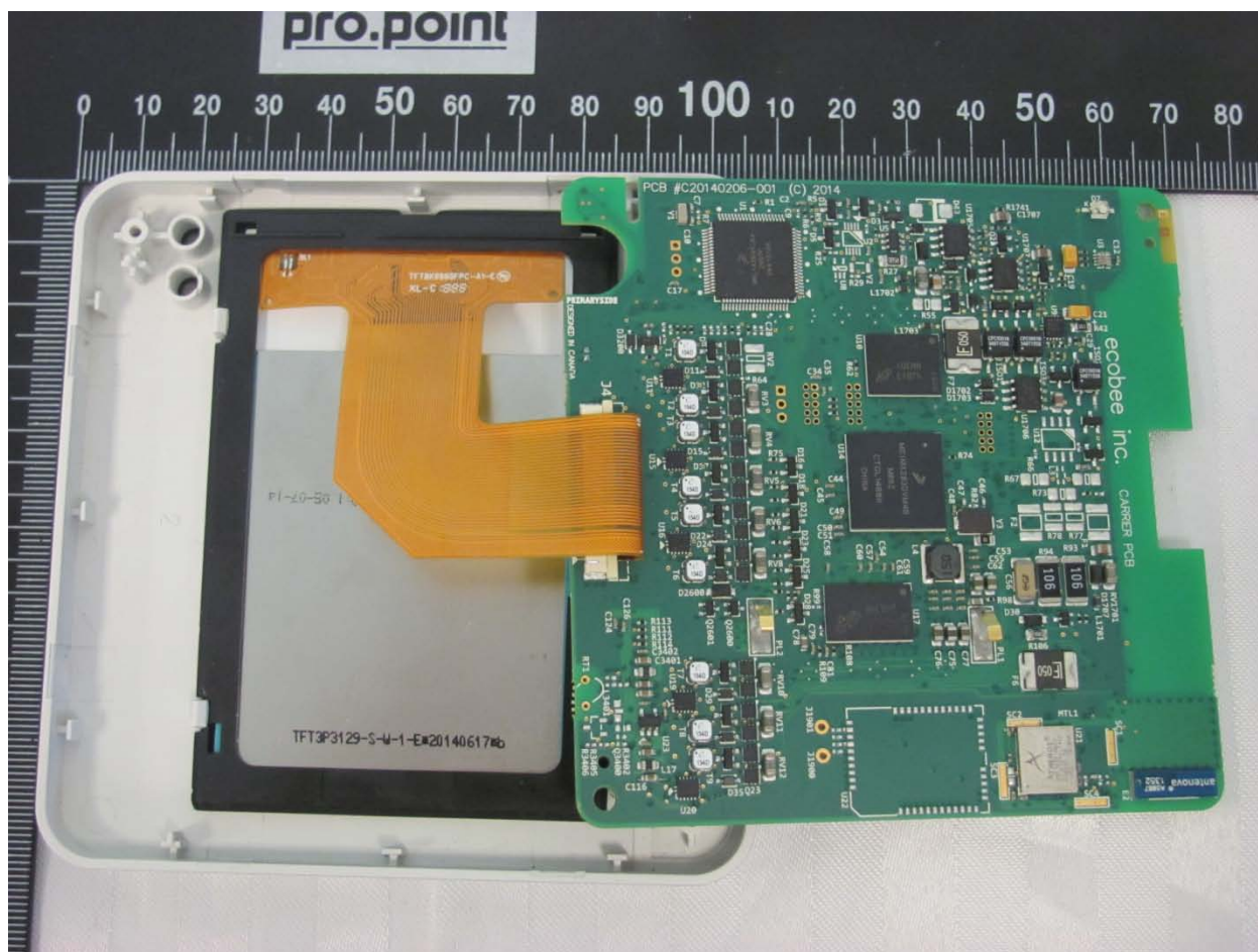
Illustration 3: EUT internal view – photo 3
