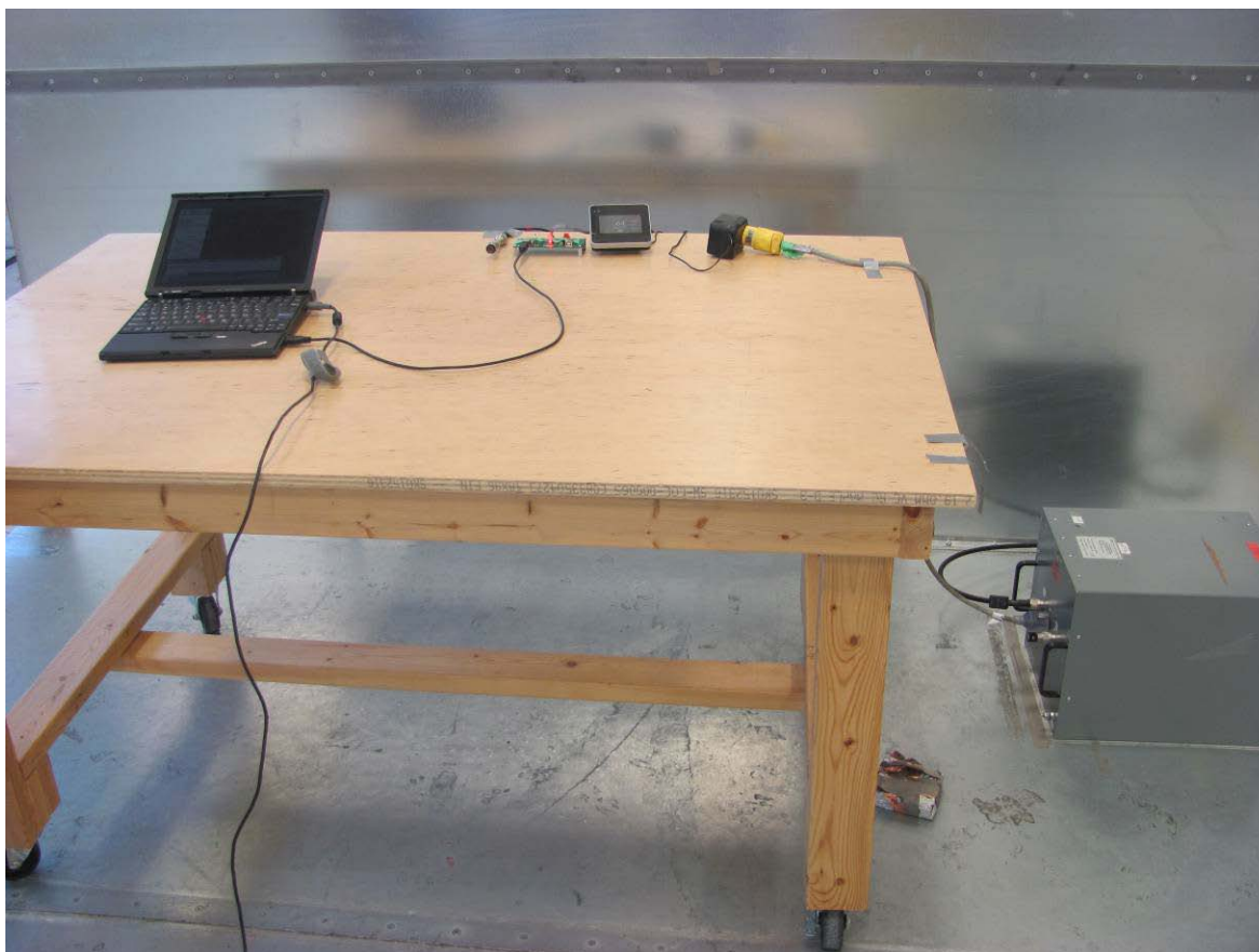
Figure 8: Power line conducted emission setup – photo 1
