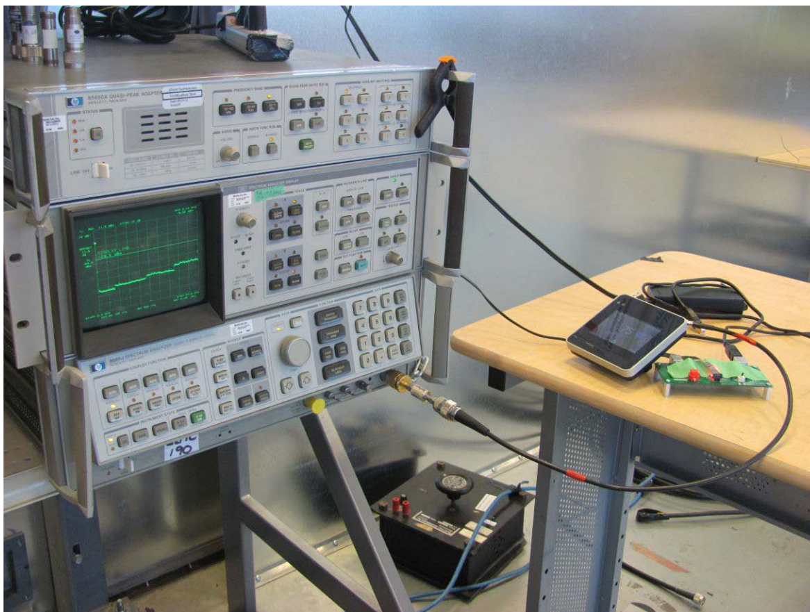
Figure 7: Antenna port conducted emission setup – photo
