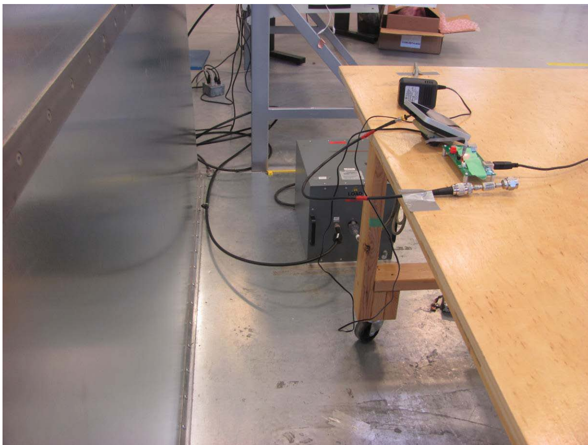
Figure 9: Power line conducted emission setup – photo 2
