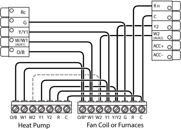
Stage 2 Heat Pump and Auxiliary Heat * Connect to O/B terminal on furnace or fan coil, if available
