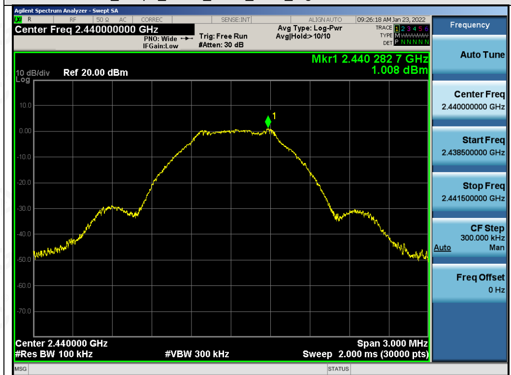
Test_Graph_GFSK_ANT1_2440_Reference Level
