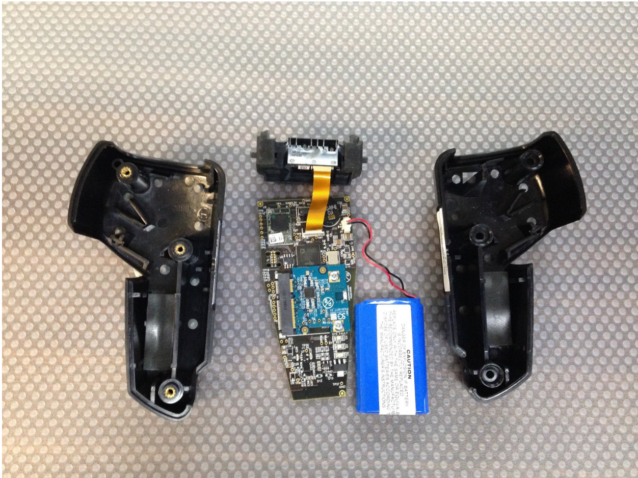
Figure 5. Host Device- Blow Up of Internal Parts
