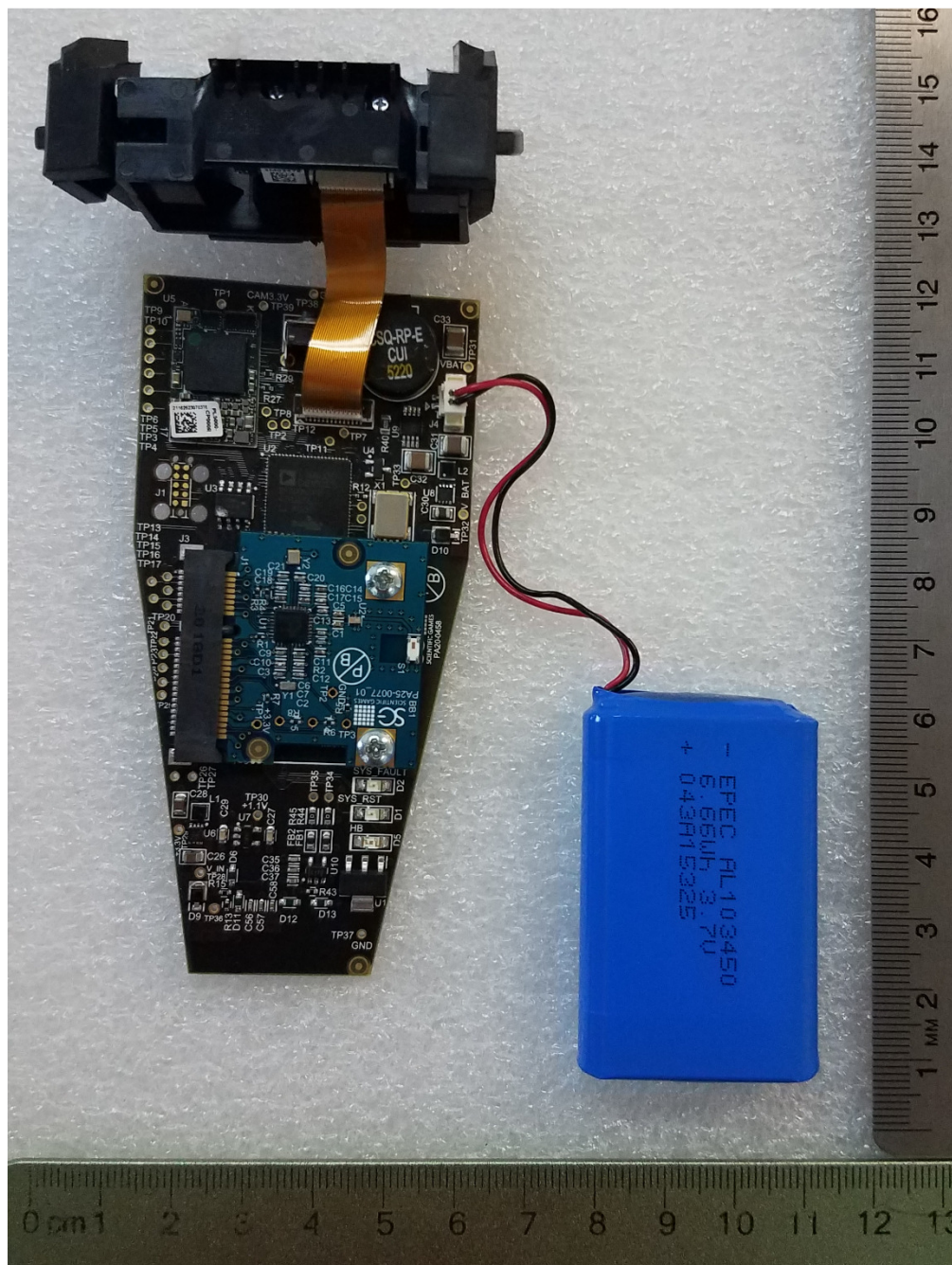
Figure 1. Radio module install on Host Device PCBA
