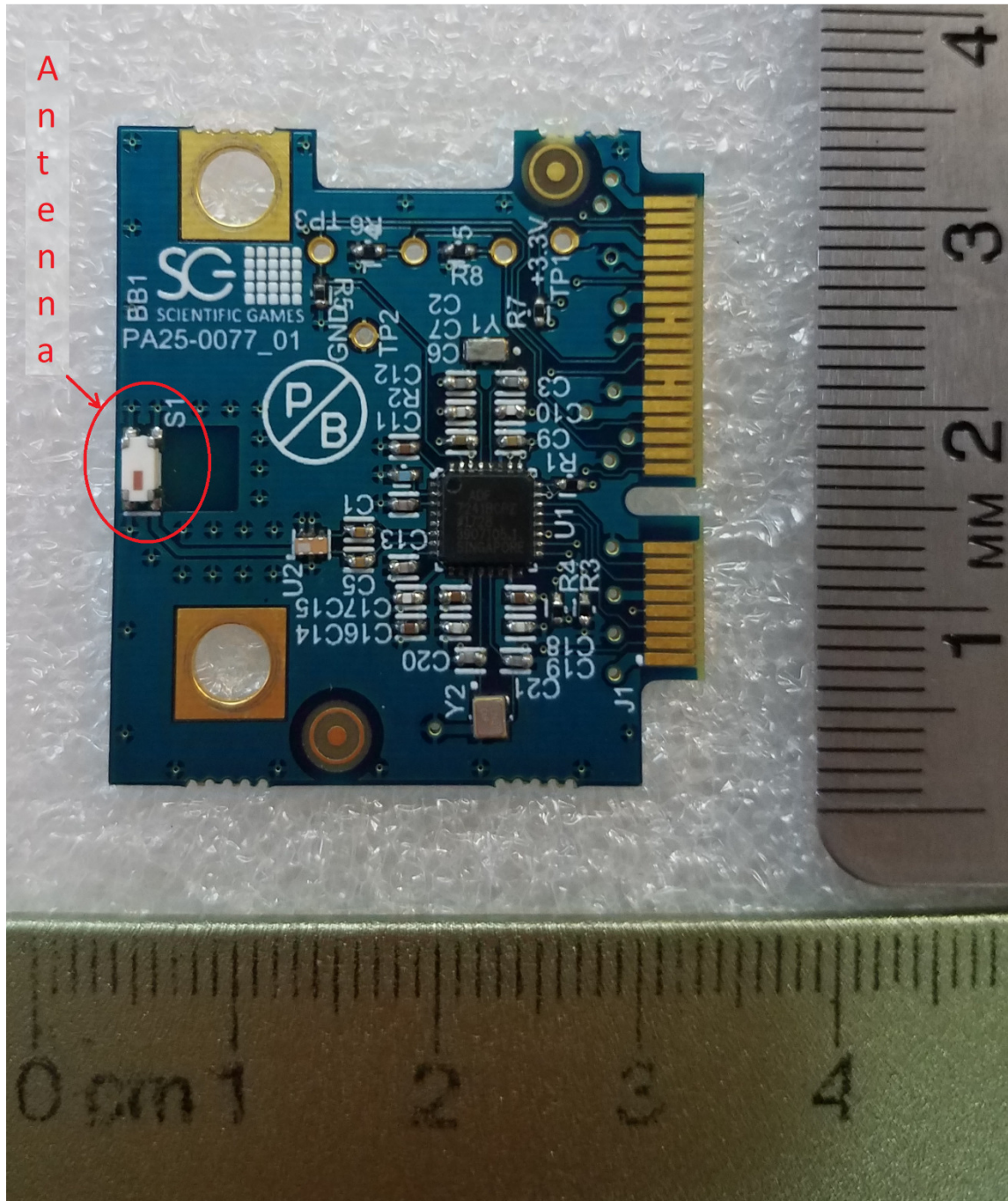
Figure 2. Front of Radio Module
