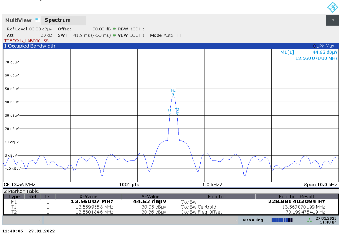
Plot No. 8: 99% Occupied bandwidth
