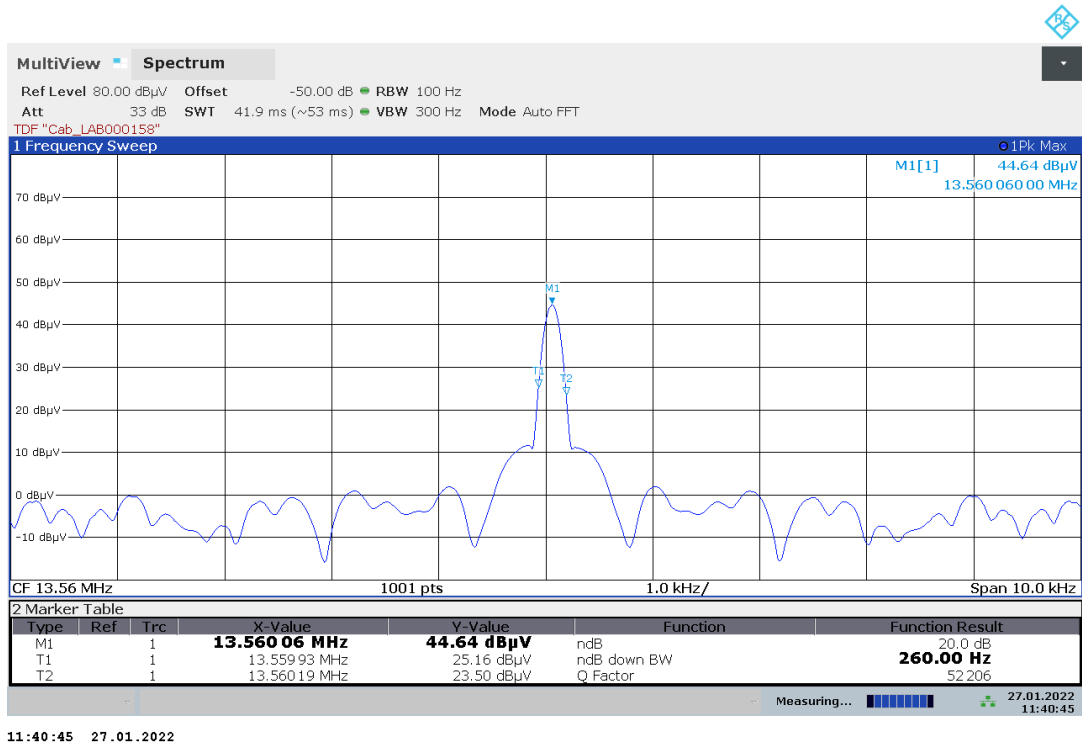
Plot No. 9: 20 dB bandwidth
