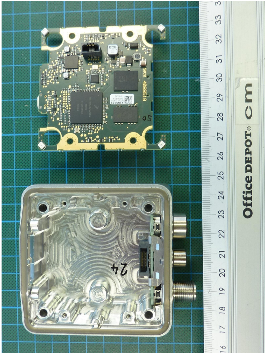
181673_fl.jpg: RFU610-10601, internal view 3, EK-Digital PCB removed
