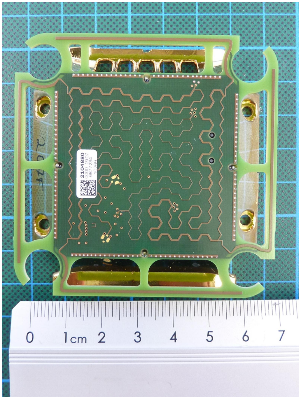
181673_fj.jpg: RFU610-10601, EK-Frontend PCB, top view
