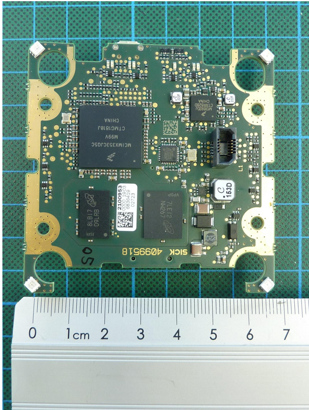
181673_fn.jpg: RFU610-10601, EK-Digital PCB, top view
