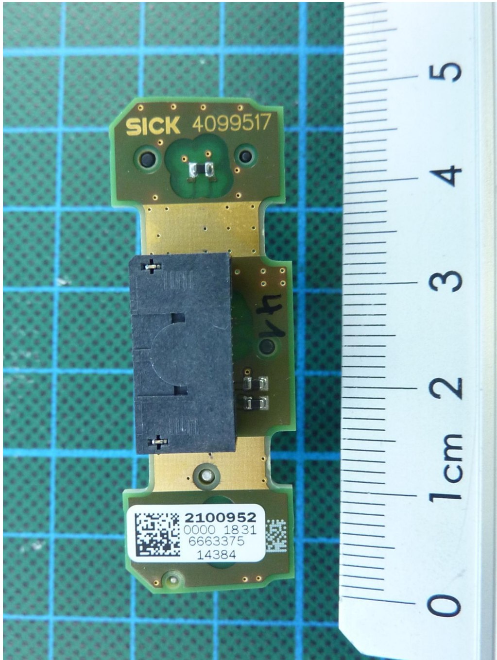
181673_fp.jpg: RFU610-10601, EK-Koppler PCB, bottom view
