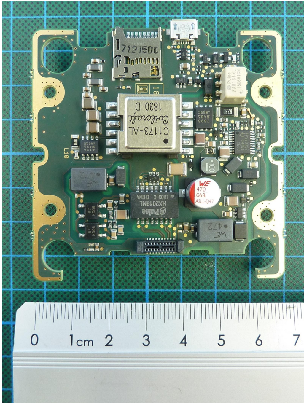
181673_fm.jpg: RFU610-10601, EK-Digital PCB, bottom view
