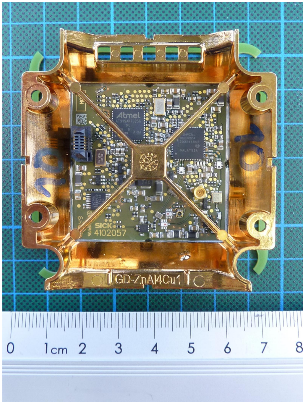
181673_fk.jpg: RFU610-10601, EK-Frontend PCB, bottom view
