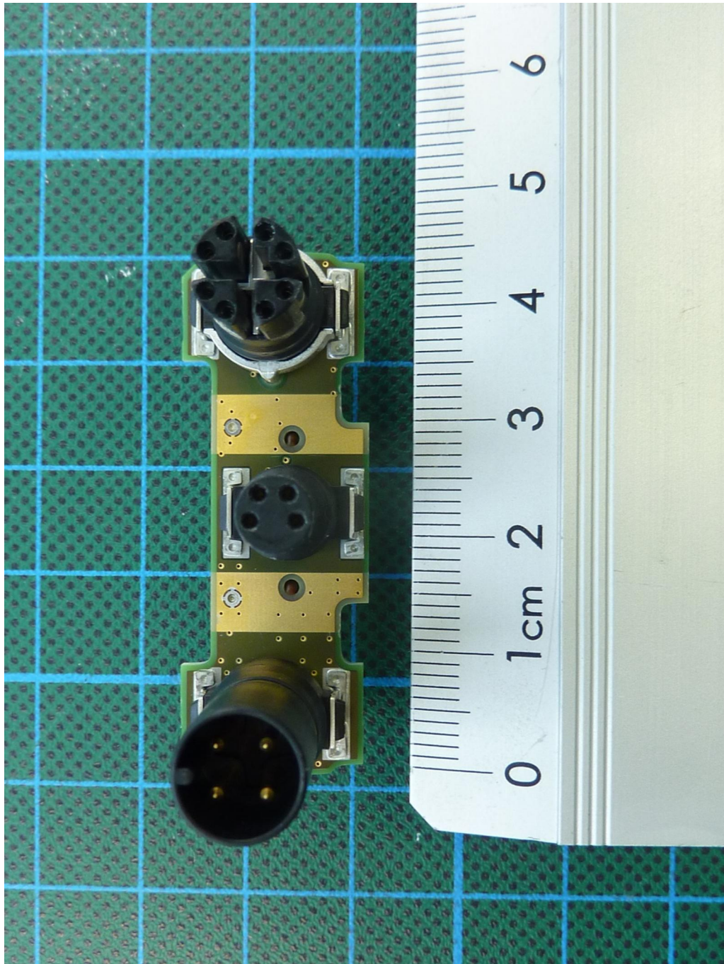
181673_fq.jpg: RFU610-10601, EK-Koppler PCB, top view
