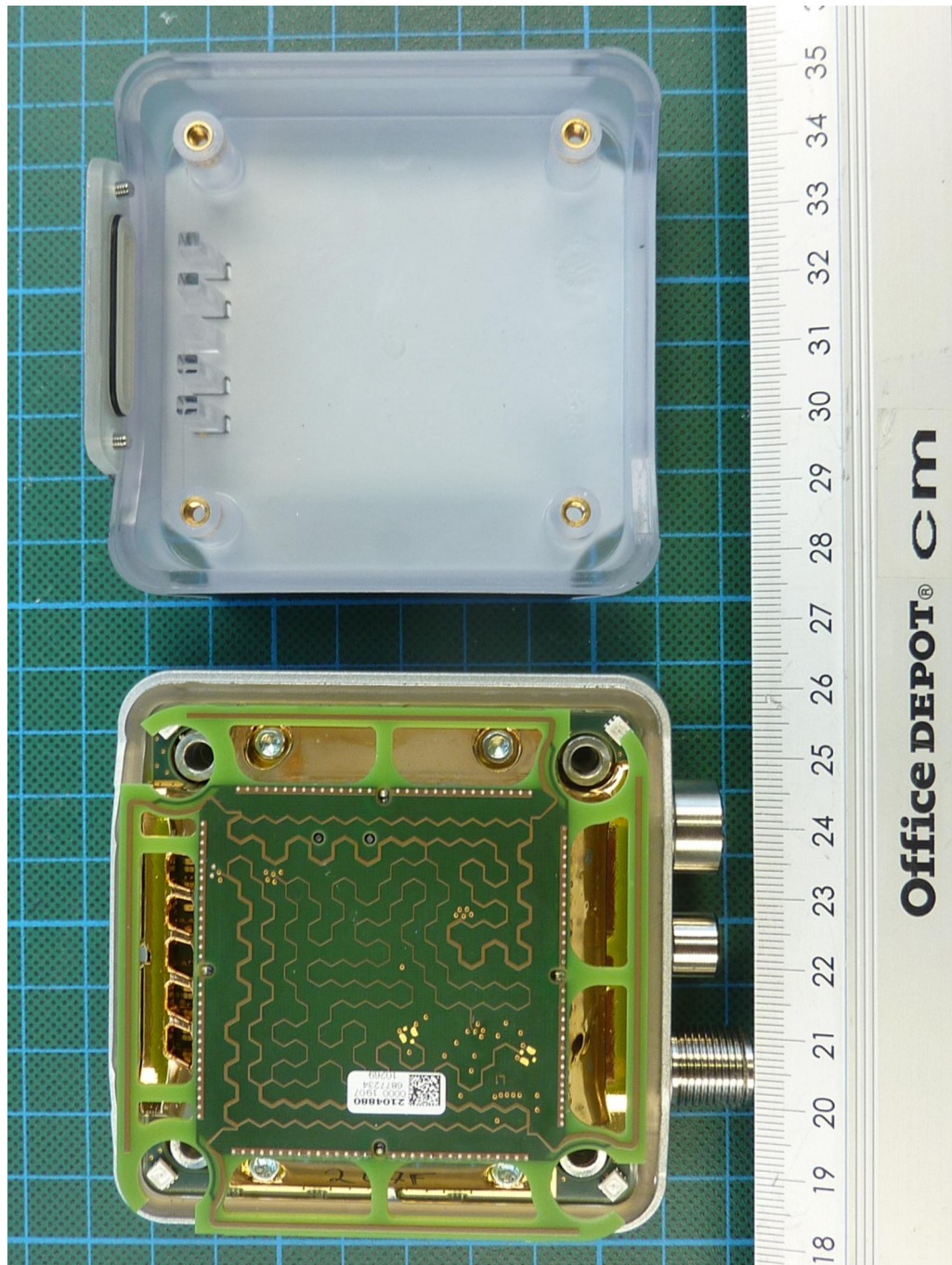
181673_fh.jpg: RFU610-10601, internal view 1, housing opened
