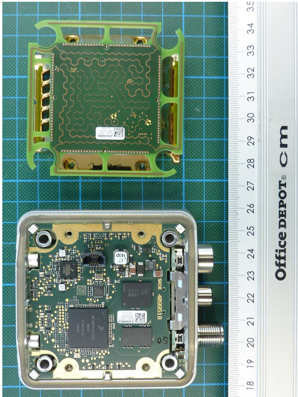
181673_fi.jpg: RFU610-10601, internal view 2, EK-Frontend PCB removed
