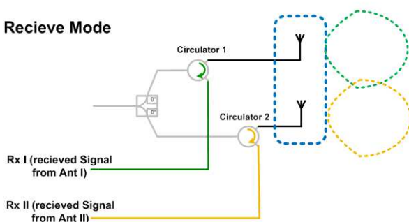
RFU 650 antenna operation modes schematic model
