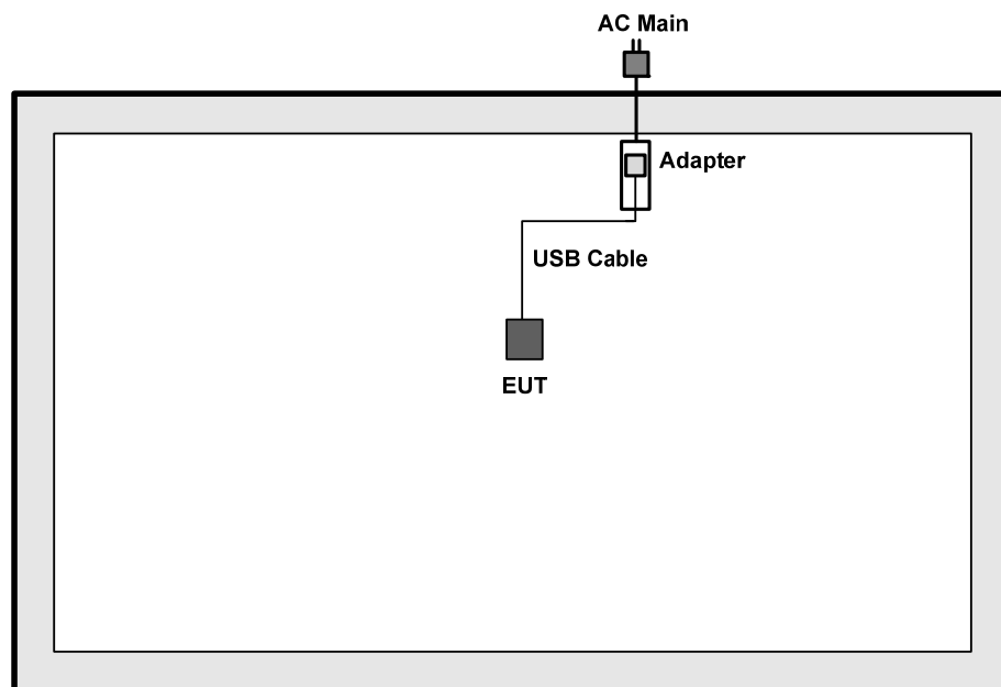
Test Setup Diagram - Radiated Emission Test Mode 2 (Above 1GHz)
