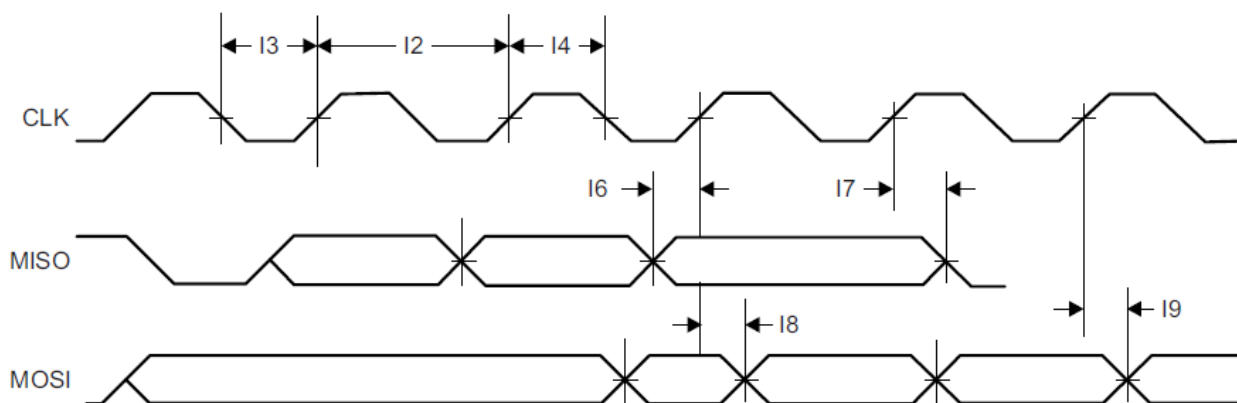
Fig 3.5.1 Host SPI interface timing
