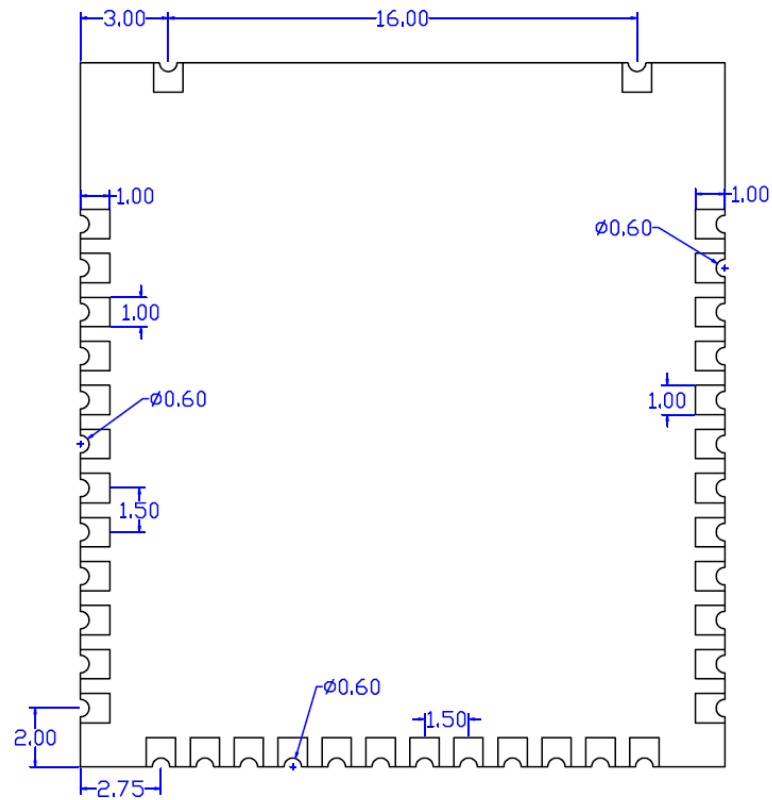
Bottom View
