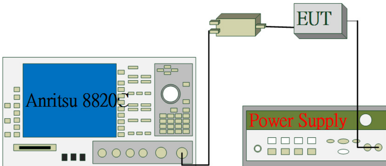
Fig. 2-1 Configuration of Tested System (Fixed Channel-Conducted & Radiated)
