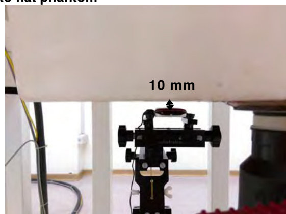
Fig.9 EUT Back side with headset to flat phantom
