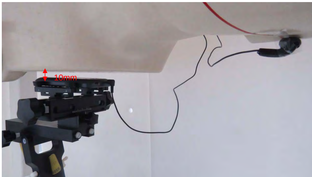
Picture 12: Back Side with Earphone 1, the distance from handset to the bottom of the Phantom is 10mm
