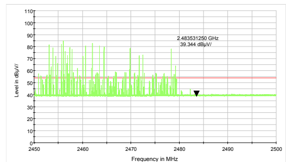
3DH5-Channel 78: Average
