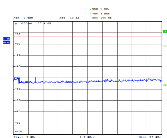
GSM 1900 CH-Low 3GHz~20GHz
