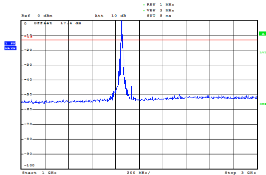
GSM 1900 CH-Low 1GHz~3GHz
