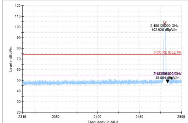
Bandedge (High): GFSK, high channel
