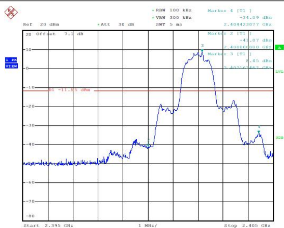
Frequency Band Edge: 8DPSK, Ch0, Hopping OFF
