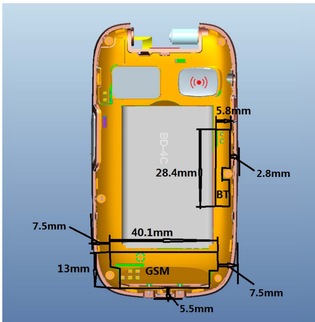
Picture 5: Constituents of EUT
