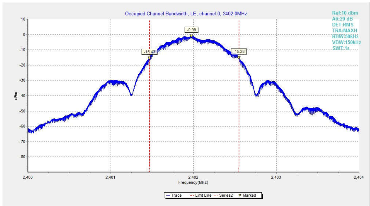
Fig.28 Occupied Bandwidth: GFSK, Channel 0
