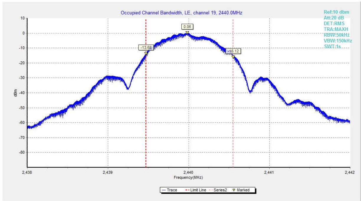
Fig.29 Occupied Bandwidth: GFSK, Channel 19
