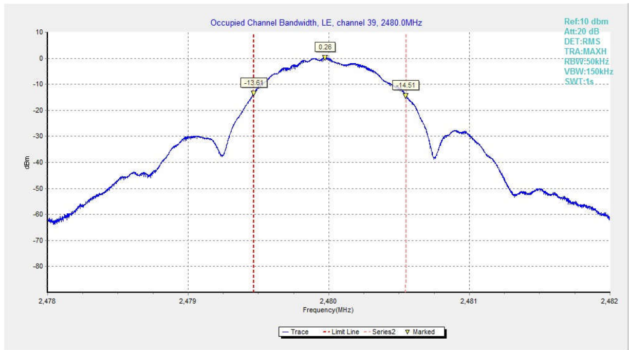
Fig.30 Occupied Bandwidth: GFSK, Channel 39
