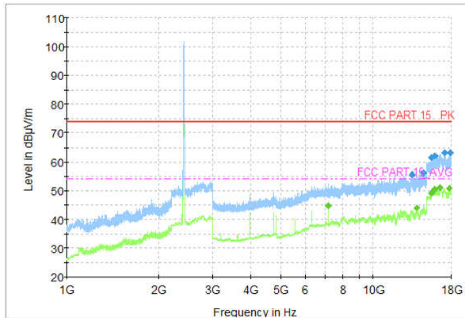
Fig.34 Radiated Spurious Emission (802.11b, CH1, 1 GHz-18GHz)
