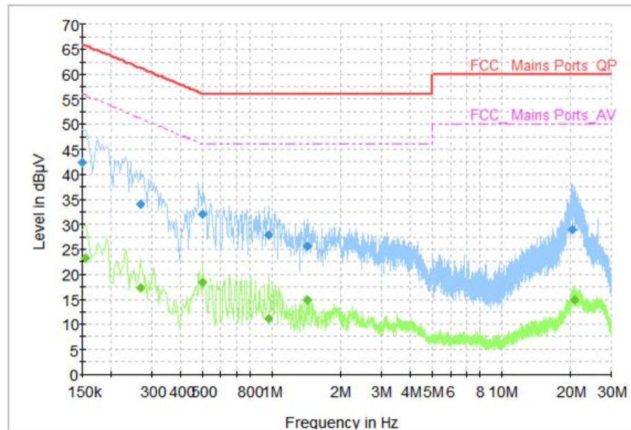
Fig. 75 AC Power line Conducted Emission (Traffic)
