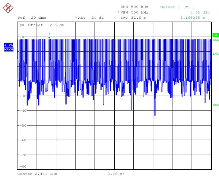
Fig.58 Time of occupancy (Dwell Time): Ch39,Packet 3-DH1
