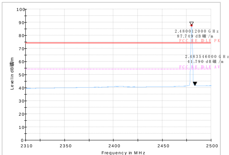
Fig.44 Bandedge (High): GFSK, high channel
