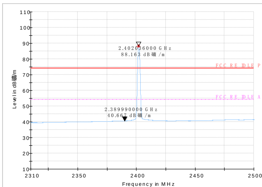
Fig.53 Bandedge (Low): 8DPSK, low channel
