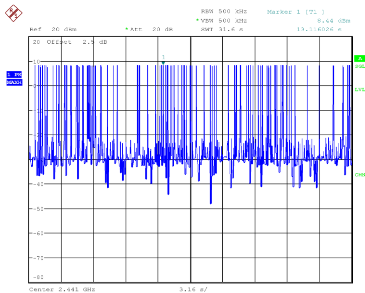
Fig.71 Time of occupancy (Dwell Time): Ch39,Packet 3-DH5
