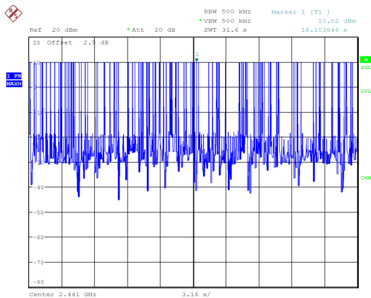
Fig.59 Time of occupancy (Dwell Time): Ch39,Packet DH5
