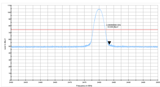
3DH5-Channel 78: Peak
