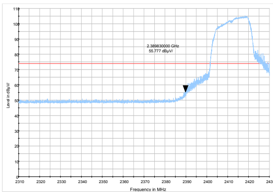
802.11g-Channel 1 Peak
